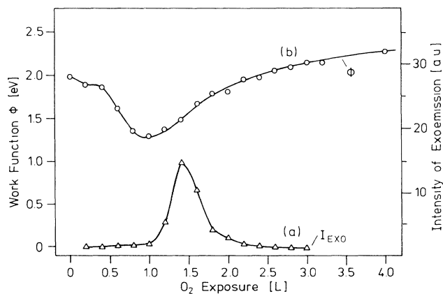
FIG. 1. Yield of exoelectrons (curve a ) and work function \phi (curve b ) of a thin Cs film as a function of O 2 exposure.
