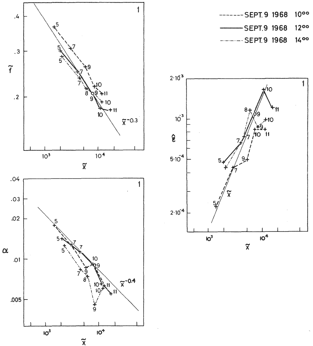
Fig. 2 A.2. Scale parameters f , z and v \cdot x for generation case 1. The dot (Station 9) denotes the position at which the source function was computed. Straight lines represent the fetch dependence used in computing the derivatives \frac{1}{\bar{x}} \frac{d}{d\bar{x}} . Estimates of the (smaller) time derivatives were obtained from neighbouring measurements taken 2 hrs. earlier and later (broken lines) than the measurements at 12 h (full line)
