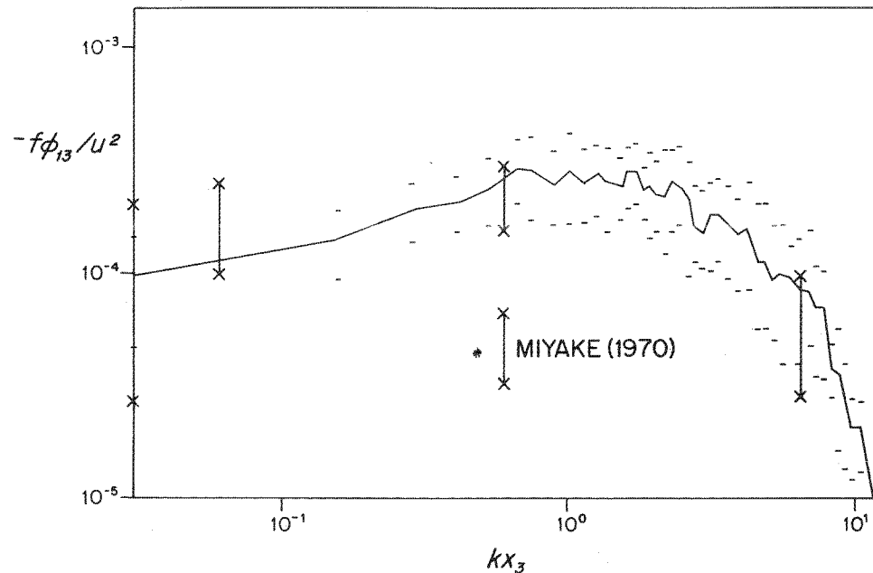
Fig. 2.2. Reynolds stress spectrum ( k = 2\pi/U_{10} , x_3 = anemometer height, U \approx U_{10} )
