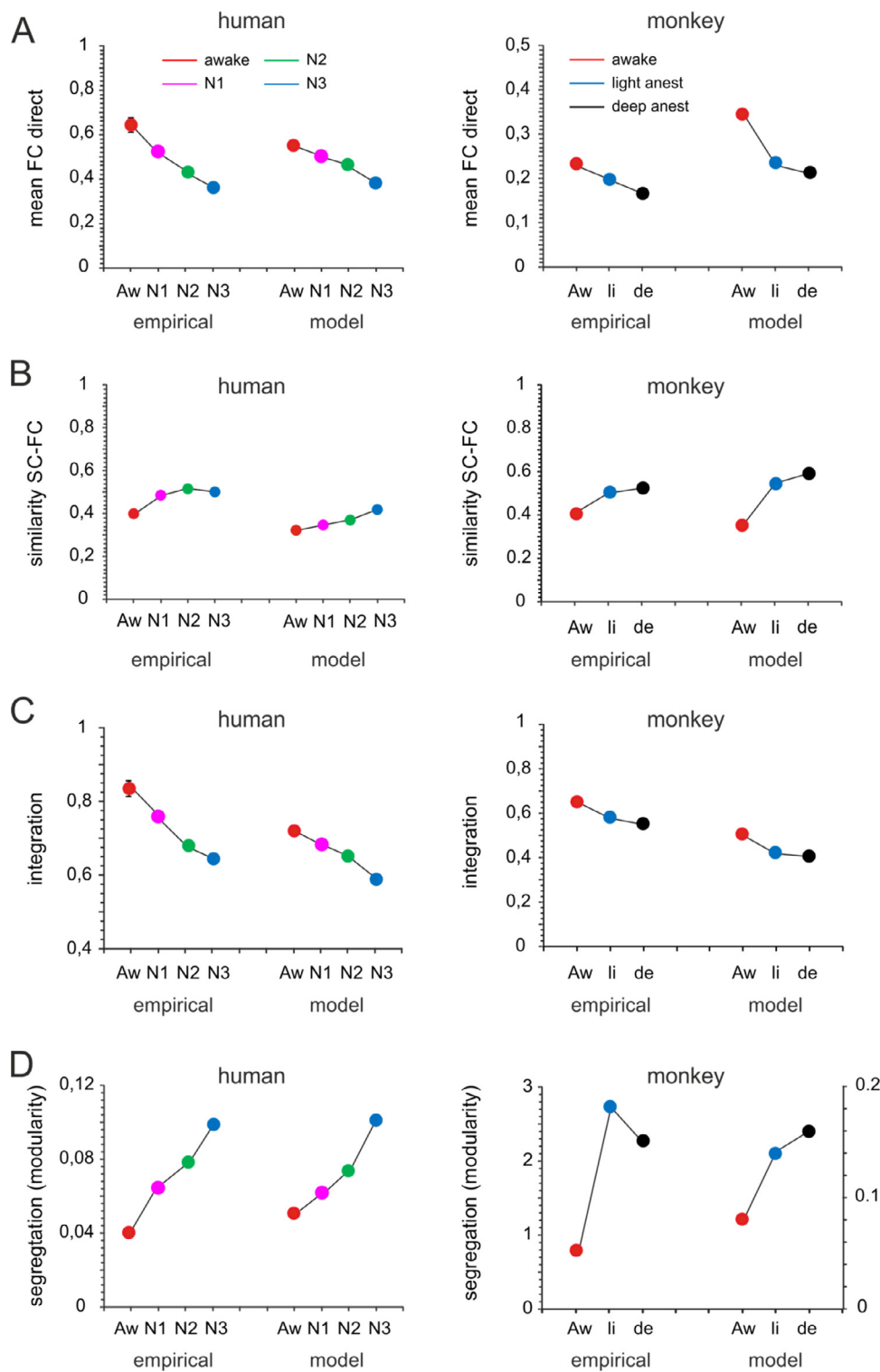
Fig. 3. Comparison between empirical data and model predictions for various measures and across different consciousness levels. (A) Mean ( \pm SD) direct FC for empirical and modeled human (left) and monkey data (right) of different consciousness conditions. (B) Same as in (A) for SC-FC similarity. (C). Same as in (A) for the level of integration. (D) Same as in (A) for the level of functional segregation as measured by modularity.
