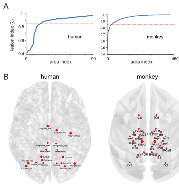
Fig. 6. Global synchronization changes after model lesions of specific brain areas. (A) The lesion index ( \lambda ) indicates the degree of global synchronization with respect to the awake state (normalized to 1) after the lesion of individual model nodes (abscissa). Dashed red line: threshold for global synchronization levels comparable to conscious (above line) and unconscious states (below line). (B) Brain areas (red circles) that cause a drop below the red line in (A) after lesion. Circle diameter is scaled to the value of the lesion index of a given area. See Supplementary Tables 1–2 for full labels.
