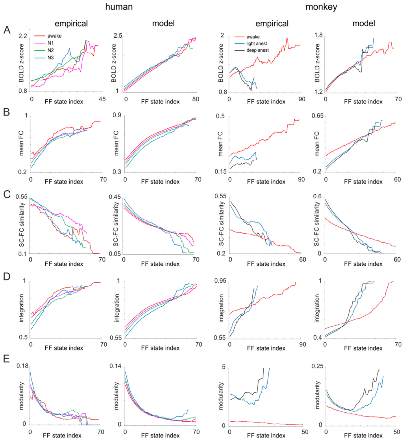
Fig. 4. Various metrics change with the level of global synchronization (FF states) across different consciousness conditions. (A) Average peak amplitude (z-score) within a time window of 5 TR as a function of FF state in empirical and modeled human (left) and monkey data (right). (B) Mean direct FC as a function of global synchronization states for human and monkey data. (C) SC-FC similarity for different global synchronization states in humans and monkeys. (D-E) Same as in (C) for integration and modularity, respectively.
