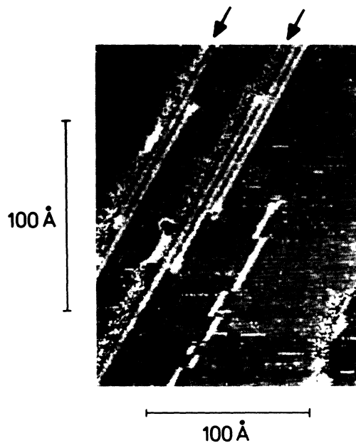
FIG. 3. STM image of (2 \times 1) O nuclei in different growth phases: two nuclei two and three rows wide, respectively, at the upper edge of steps along [001] and a single-row nucleus on the flat terrace. Step edges are marked by arrows.
