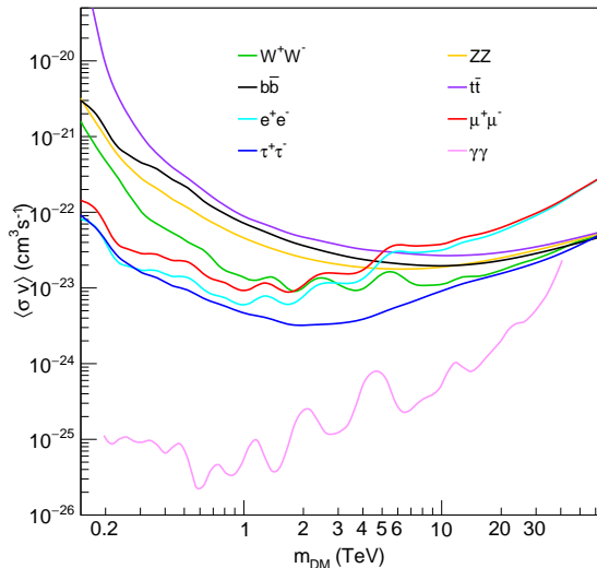
FIG. 7: Combined 95% C.L. observed upper limits on the annihilation cross section \langle\sigma v\rangle versus the DM mass m_{\text{DM}} for the combined analysis in the bb , t\bar{t} , W^+W^- , ZZ , e^+e^- , \mu^+\mu^- , \tau^+\tau^- , and \gamma\gamma annihilation channels, respectively, without the uncertainty on the J -factor.
