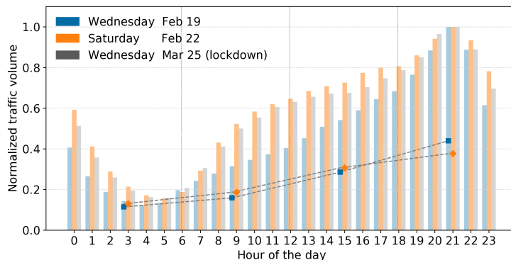
Figure 2: Workday vs. weekend patterns before and after the lockdown
