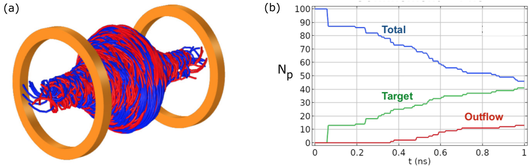
FIGURE 7. a) 3-MeV electron (blue) and positron (red) single particle paths in magnetic mirror generated by two 15-T 5-mm inner radius coils separated by 15 mm. The paths originate at target placed in the center of the mirror. b) The time evolution of 100 positrons in the mirror. The total positron number in the mirror (blue), losses due to target collisions (green), and losses due to (non-adiabatic) outflows (red).
