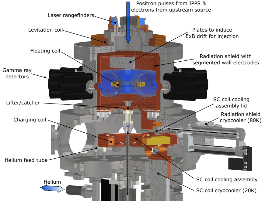
FIGURE 6. Schematic diagram of the APEX levitated dipole experiment with representative field lines and, in blue, the surface of outermost field lines that do not intersect material surfaces.
