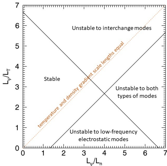
FIGURE 2. The stability landscape for pair plasma in a magnetic dipole (adapted from Fig. 1 in (Helander & Connor 2016)) showing the stability boundaries for interchange and low-frequency electrostatic modes in the space of normalized inverse temperature gradient scale length vs. normalized inverse density gradient scale length. The dashed line with unit slope indicates the contour where the temperature and density gradients are equal.
