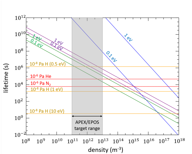
FIGURE 4. Lifetimes of positrons versus plasma density (at temperatures of 0.1 eV and 1 eV) set by direct annihilation with plasma electrons (purple), Ps formation via radiative recombination (green) and via three-body recombination (blue); lifetimes for positrons set by direct annihilation on atomic/molecular electrons (in red, for two gas composition and pressure values), and by Ps formation via charge exchange on atomic hydrogen at various plasma temperatures (yellow). The anticipated experimental range for low-density magnetically confined plasma experiments is indicated in gray. This figure is adapted from similar figures in Greaves & Surko (2002) and Saitoh et al. (2014).
