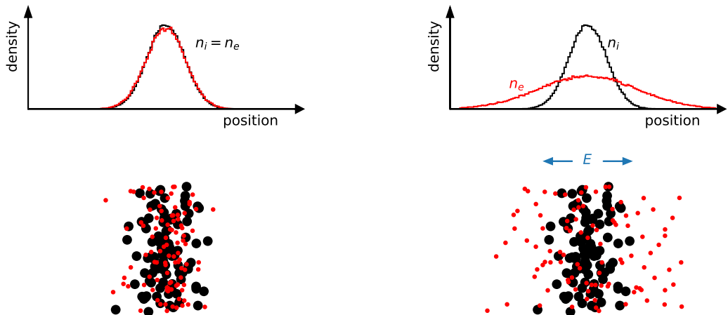
FIGURE 1. Creation of an ion acoustic wave from a density perturbation in a conventional (electron-ion) plasma. As the electrons flow out of the region of increased density faster than the ions, an electric field is produced. The ions collectively accelerate in this self-produced field, which leads to an ion density wave. In an electron-positron plasma, the physics of this wave is greatly modified.
