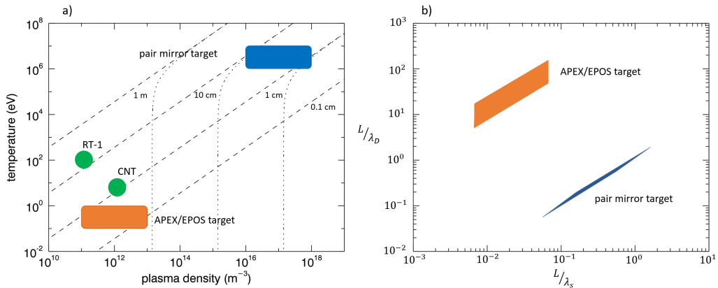
FIGURE 3. a) Target parameters (temperature and density) for pair plasma experiments discussed in this paper: low-density magnetically confined plasmas (orange) and relativistic laser-produced plasmas (blue). Also shown are achieved parameters for non-neutral plasmas in a levitated dipole (RT-1) and a stellarator (CNT). The contours indicate the Debye length (long dash) and skin depth (short dash) at each combination of density and temperature. b) Planned operating regimes of the relativistic pair mirror (blue) and low-density (low-temperature) magnetically confined pair plasma (orange) in terms of the plasma size, L , as a ratio of the Debye length, \lambda_D , versus as a ratio of the skin depth, \lambda_s .
