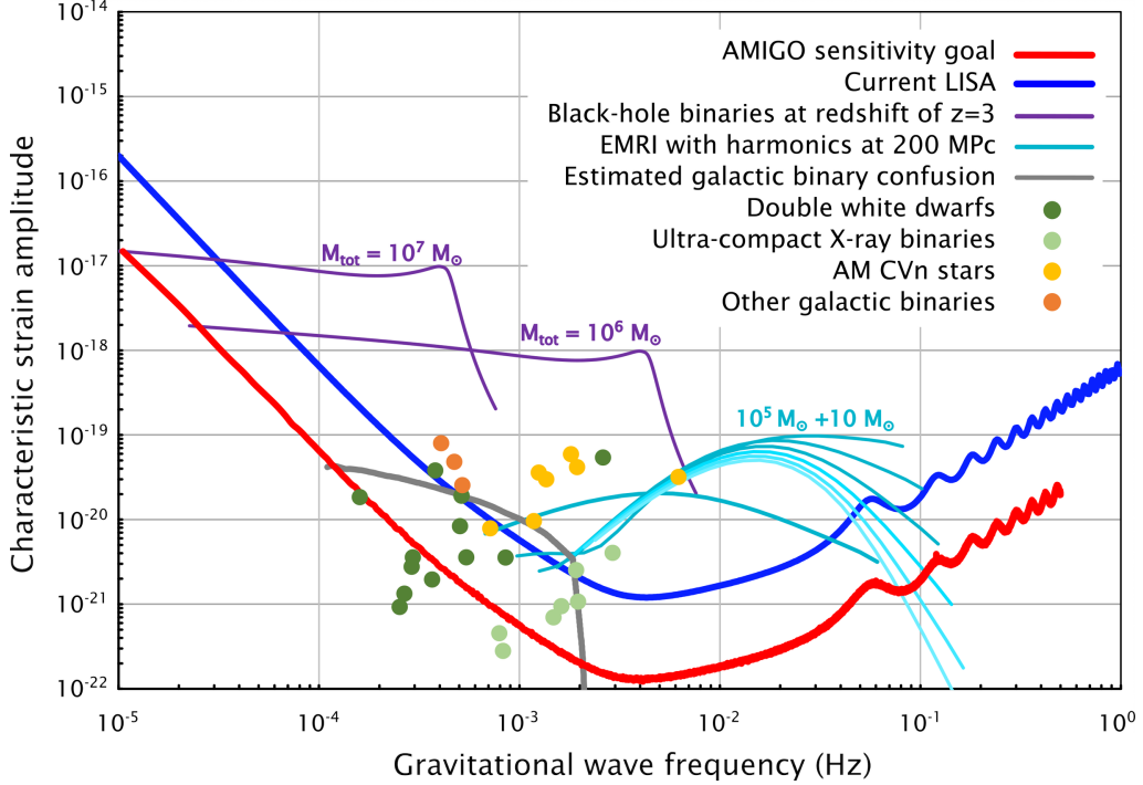
Figure 1: Projected sky-averaged sensitivity curve for AMIGO and possible sources within its range [18]. The sensitivity curve was computed with the use of the LISA Performance Model ( perf-lisa.in2p3.fr ) and the sources were adapted from [19].
