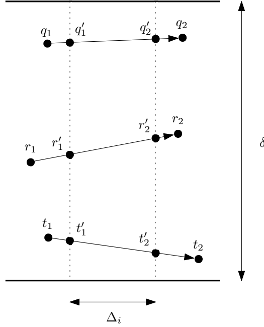
Figure 12 An example of Lemma 16, with k = 2 . Suppose |q_1q_2| + |r_1r_2| < |q_1r_1| + |q_2r_2| and |r_1r_2| + |t_1t_2| < |r_1t_1| + |r_2t_2| . Since \delta \geq |q_1'q_2| + |r_1't_1| and \delta \geq |q_2'r_2| + |r_2't_2| , we get that 2\delta \geq |q_1'r_1| + |q_2'r_2| + |r_1't_1| + |r_2't_2| > |q_1'q_2| + 2|r_1'r_2| + |t_1't_2| \geq 4\Delta_i .
