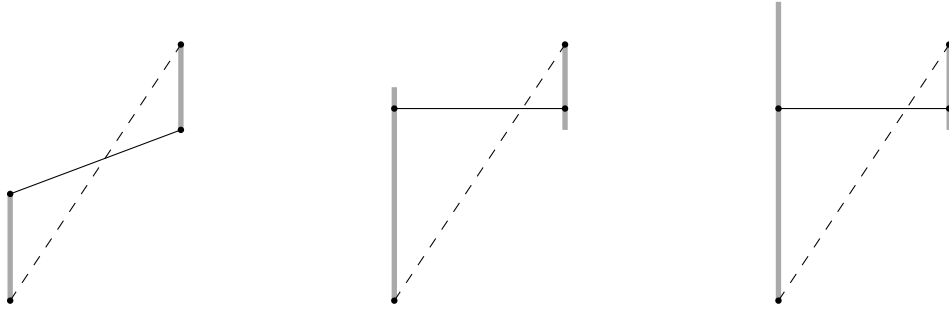
■ Figure 9 Three pairs of intervals, the shortest edges between points in those intervals (solid) and the longest edges between points in those intervals (dashed)
