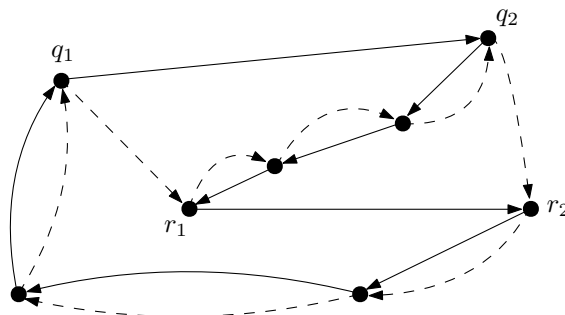
■ Figure 10 Illustration of Observation 14. T is the solid line, T' is the dashed line. Between x(r_1) and x(q_2) , the tonicity of T' is 2 lower than the tonicity of T .
