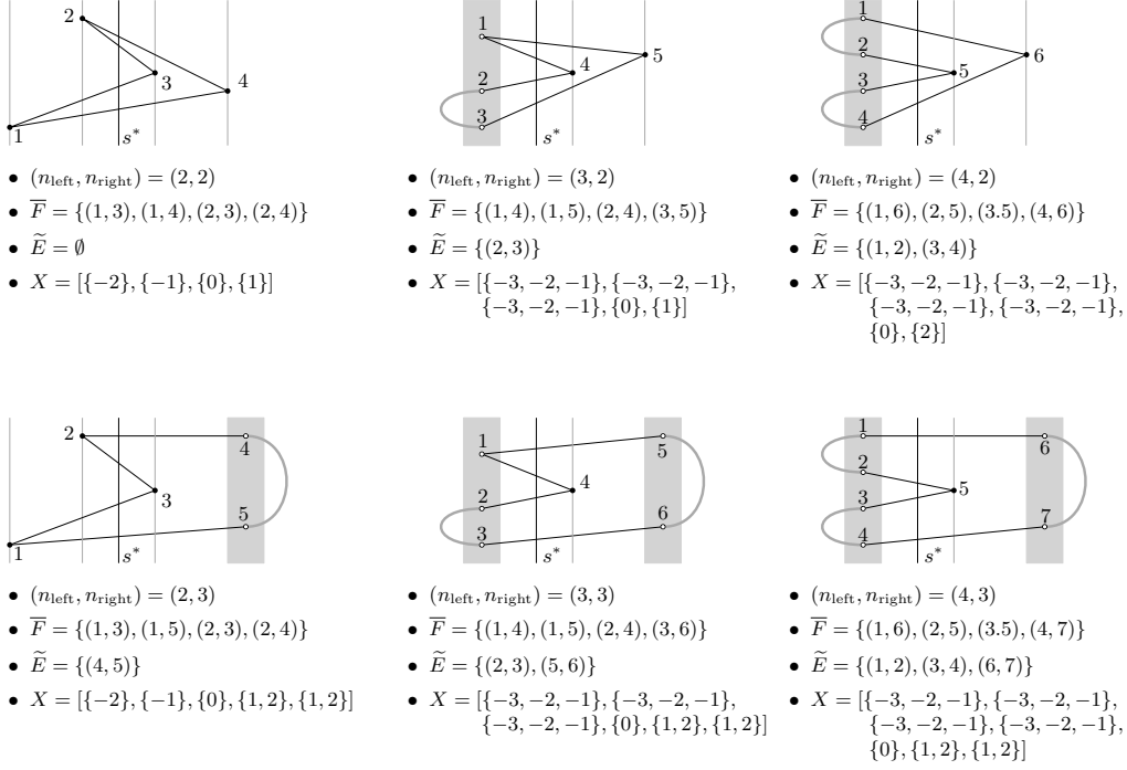
■ Figure 4 The six different cases that result after applying Step 1 of the proof. Points indicated by filled disks have a fixed x -coordinate. The left-to-right order of points drawn inside a grey rectangle, on the other hand, is not known yet. The vertical order of the edges is also not fixed, as the points can have any y -coordinate in the range [0, 2\sqrt{2}] .
