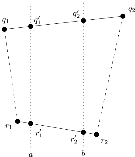
■ Figure 11 Illustration of Observation 15. Since |q_1q_2| + |r_1r_2| < |q_1r_1| + |q_2r_2| holds, |q'_1q'_2| + |r'_1r'_2| < |q'_1r'_1| + |q'_2r'_2| also holds.
