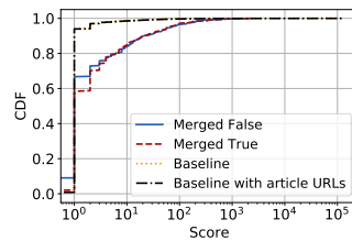
Figure 12: CDF of Reddit submission score on submissions sharing news articles.
