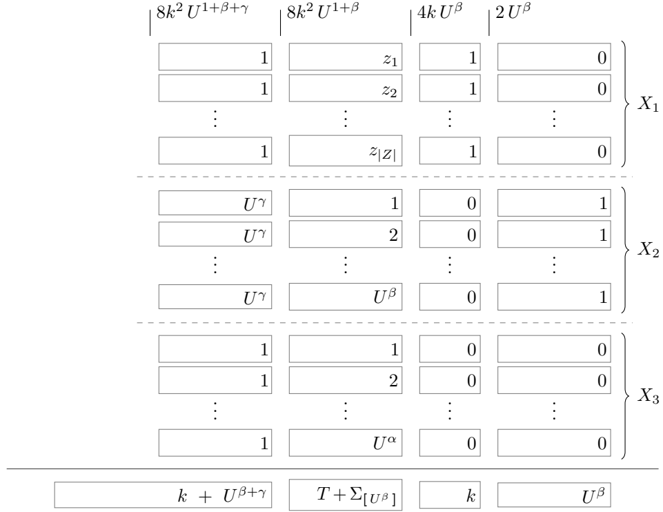
Figure 1 An overview over the reduction from k -Sum to Subset Sum. The given k -Sum instance is (Z, T) , and we write Z = \{z_1, \dots, z_{|Z|}\} . Bit blocks of the constructed numbers are depicted as boxes, the value of a bit block is written inside the corresponding box. The constructed target number is visualized at the bottom. The annotations at the top represent the maximum value of the constructed numbers up to the specified point. The annotations on the right denote group of constructed numbers. We remark that the number T + \Sigma_{\lfloor U^\beta \rfloor} not necessarily fits in its block, but this is the only overflow that can occur in this figure.
