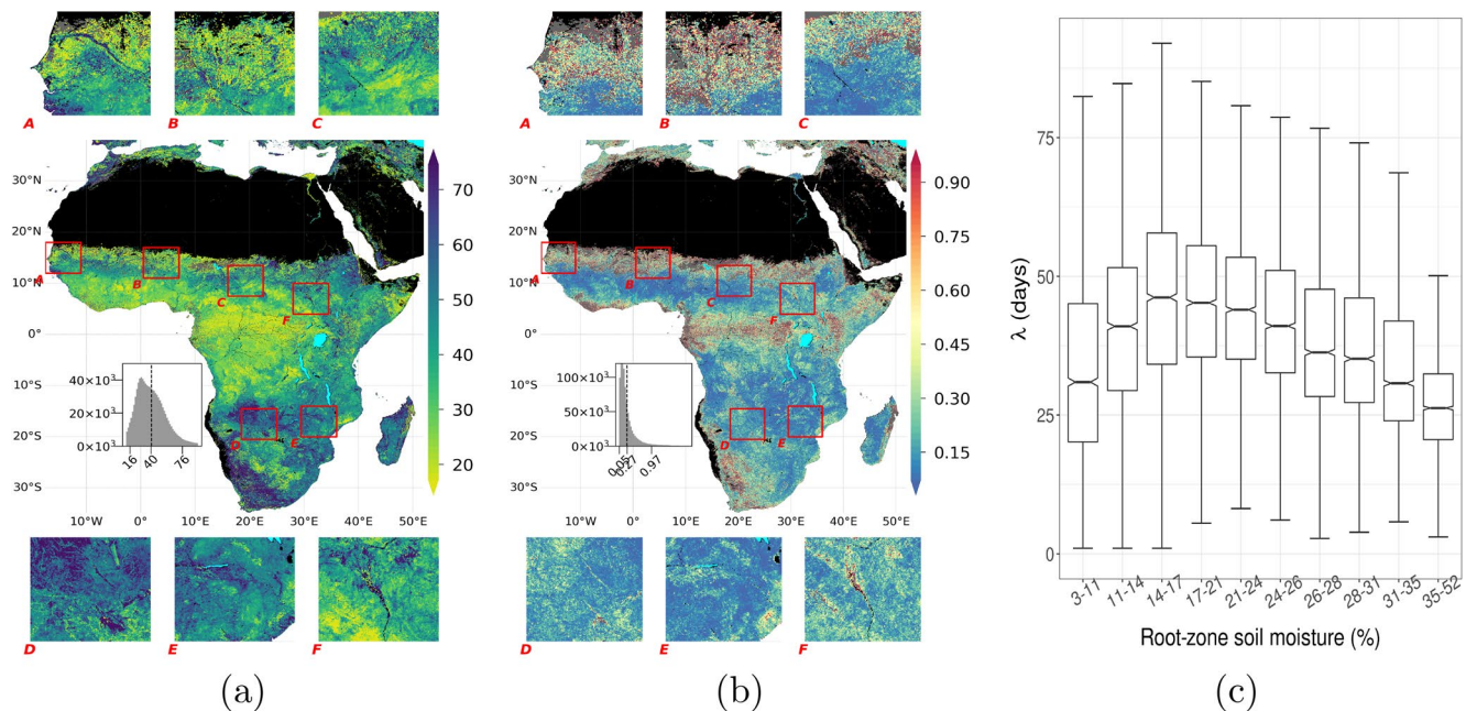
Figure 5. (a) e -folding time of FVC time series during dry-down (in days), \lambda , (b) variation of \lambda , and (c) distribution of \lambda within soil moisture. See Figure 2 for plotting details.
