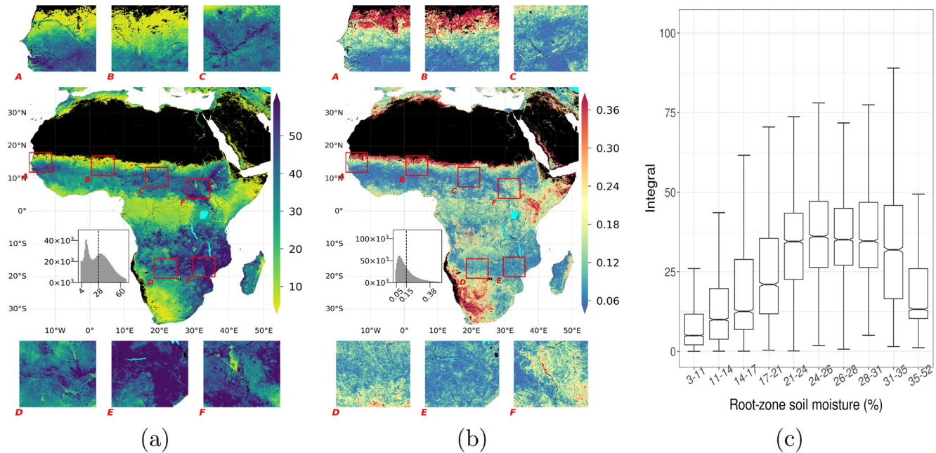
Figure 4. (a) Integral of FVC time series in the decay period, I_{dp} , (b) variation of I_{dp} , and (c) distribution of I_{dp} within mean annual soil moisture. See Figure 2 for plotting details.
