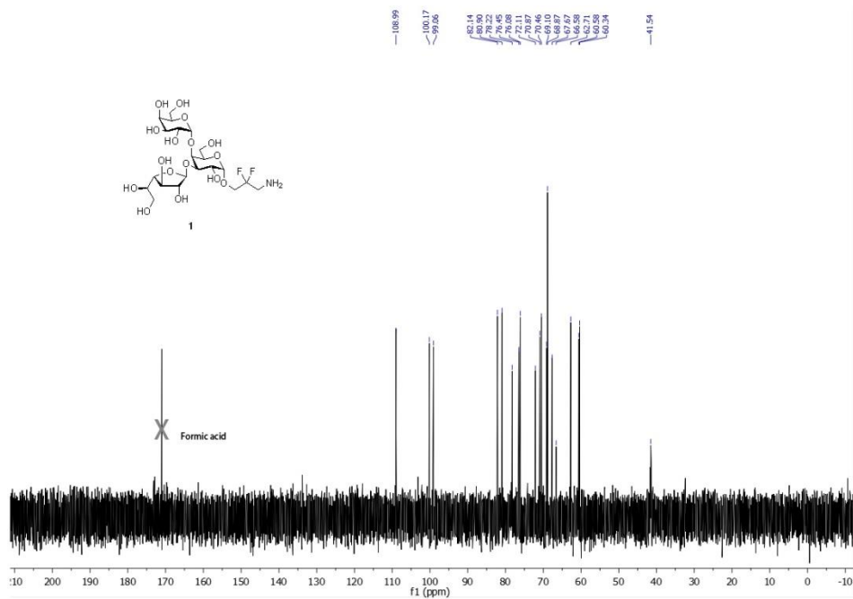
13 C NMR of 2-1
