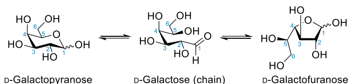
Scheme 2 Cyclization of acyclic D-galactose to form pyranose and furanose structures Cyclization reactions usually produce both \alpha and \beta anomers.
