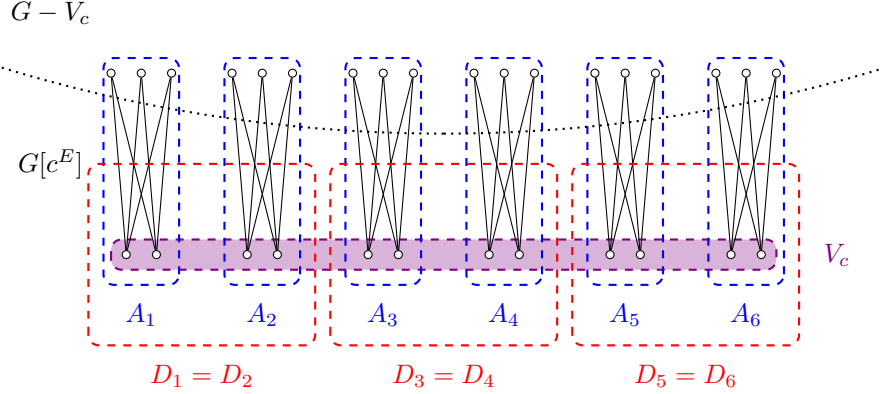
Figure 4.1: Visualization of the proof in the case s(c^E) \geq ah^3 (this condition is omitted for visualization purposes). The figure shows the part G[c^E] with six connected components A_1, \dots, A_6 . Moreover, D_1 = D_2 , D_3 = D_4 and D_5 = D_6 , and \mathcal{A}_1 = \{1, 2\} , \mathcal{A}_2 = \{3, 4\} and \mathcal{A}_3 = \{5, 6\} .
