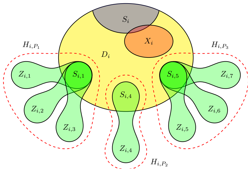
Figure 5.1: Visualization of the graph decomposition.
