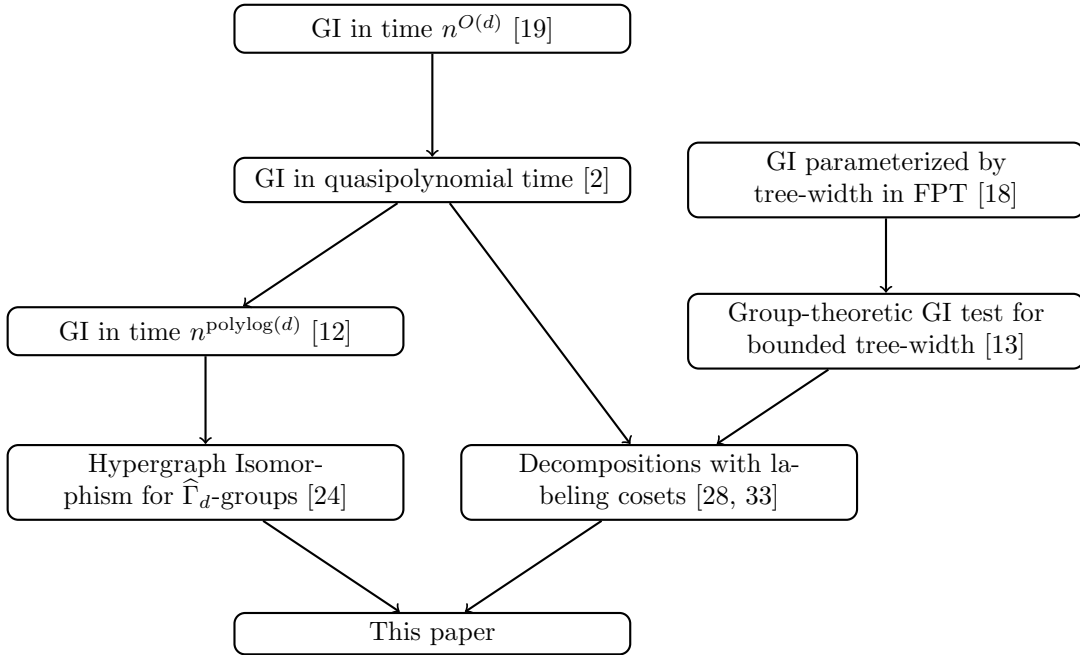
Figure 3.1: Dependencies between the main results leading to this paper.
