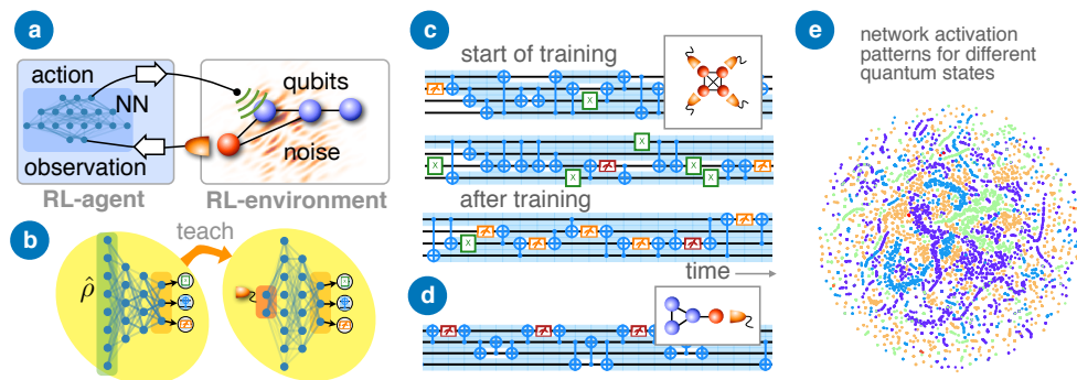
Figure 7: Discovering quantum error correction strategies from scratch [48]. (a) The setting: A neural-network-based agent controls a few qubits, applying quantum gates and measurements, with the aim of protecting the quantum information against noise. (b) RL is used for training a powerful first network that receives the quantum state \hat{\rho} as input at every time step. This is then used for supervised training of a second network that only obtains the measurement results and which can be deployed in an experiment. (c,d) Quantum circuits (i.e. action sequences) for two different qubit setups. The network learns to encode the quantum information, apply periodic collective measurements (parity detection), and eventually also to correct any errors. (e) Visualization of the network activation patterns. Each point corresponds to one quantum state (reached at a particular time, in one of many trajectories). Its location is a 2D nonlinear projection (using the t-SNE method [49]) of the high-dimensional vector of neuron activations obtained in the network for that quantum state. Different clusters (colored according to the action suggested by the network) belong to quantum states that are considered qualitatively different by the network. Using t-SNE with a higher 'perplexity' parameter (here: 30) results in more clearly separated clusters, see [48].
