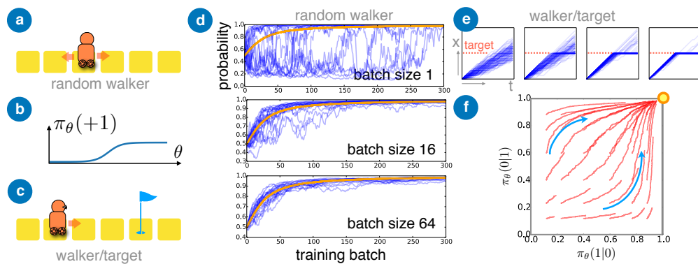
Figure 4: Simple illustrations of reinforcement learning. (a) A random walker moving either left or right in each time step, where the reward will be determined according to the distance covered to the right. (b) Dependence of the probability \pi_\theta(+1) for moving right on the policy parameter \theta . (c) The walker/target example, where the walker has to learn to stop when on target. (d) Learning progress for the random walker, using policy gradient: we display the probability to move right (which should ideally converge to 1). Increasing batch sizes lead to smoother learning behaviour. (e) Walker/target example, with a sample of trajectories x(t) , displayed for increasing learning progress (from left to right). Eventually, the walker learns to stop on target (rightmost panel). In this plot, the target was always placed at the same location x , though it has random locations during training. (f) Training evolution of the probabilities to move when not on target, \pi_\theta(1|0) , and to stop when on target, \pi_\theta(0|1) . The fixed point is indicated, representing the optimal policy.
