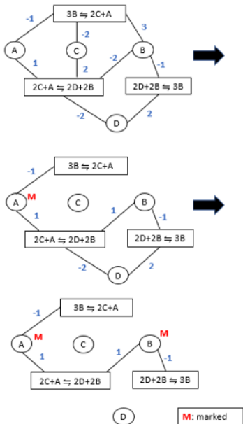
Figure 2: Algorithm 1 on Example 3.
