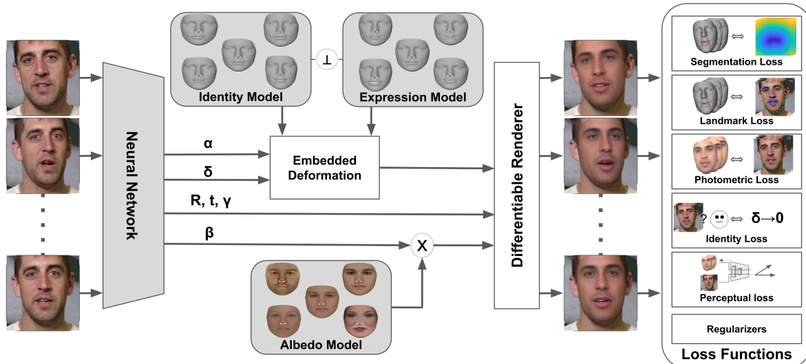
Figure 2. Our approach jointly learns identity, expression and albedo models along with the input-dependent parameters for these models. The network is trained in a siamese manner using differentiable renderer to compute self-supervised loss.
