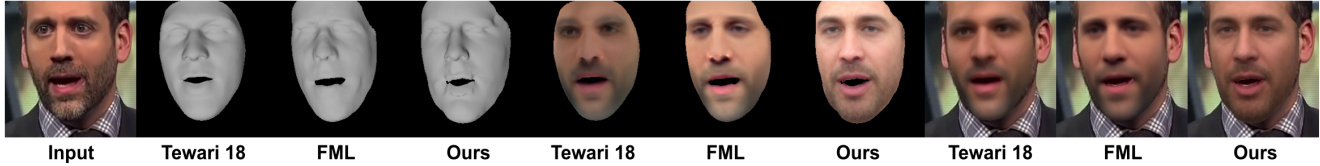
Figure 7. Our approach produces better geometry, including detailed mouth shapes compared to Tewari et al. [53] and FML [51]. Our albedo is also more detailed and better disentangled from the illumination.
