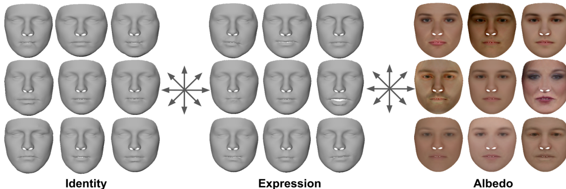
Figure 5. Visualization of learned models. Faces in each direction of indicated arrows is obtained by linearly scaling individual component of respective models. Identity geometry captures variations in face shape (second column), lips (top left to bottom right) and jaw (top right to bottom left), while expressions capture variations due to mouth opening (second row), smile (second column) and eye movement (top right to bottom left). Albedo spans a variety of skin color (second column), eye color (top right to bottom left) and gender specific features e.g. facial hair, make-up (second row).
