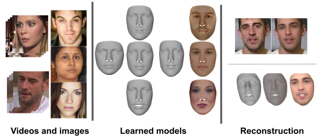
Figure 1. We present the first approach for learning complete 3D morphable face models from in-the-wild images. Our approach learns models for identity geometry, expression and albedo, completely in a self-supervised manner. It achieves good disentanglement of the various facial components and produces high quality photorealism in the final overlay.
