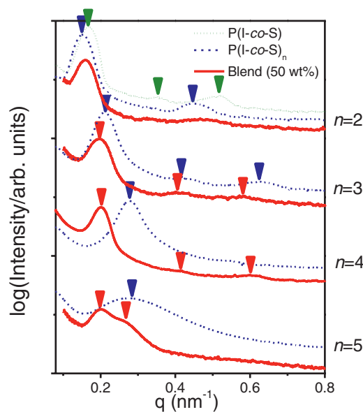
Figure 6. SAXS patterns for the P(I-co-S) (green dotted line), P(I-co-S) n copolymers ( n = 2–5; blue dashed line) and the corresponding binary symmetric (50 wt%) blends (red lines) (from entry 2 in Table 3). The curves have been shifted vertically for clarity. Arrows give the positions of the Bragg peaks corresponding to a lamellar morphology.
