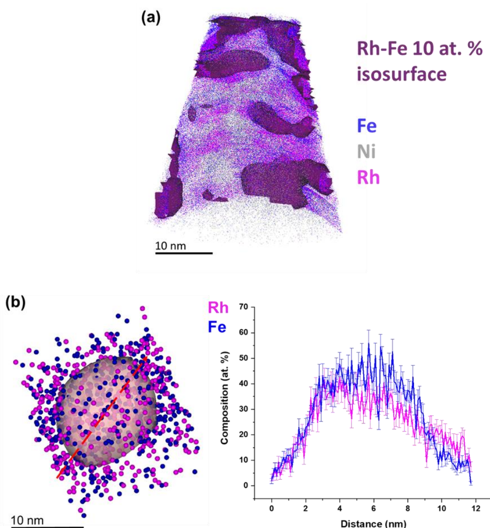
Figure 5. Atom probe tomography of FeRh nanoparticles synthesized in acetone and argon atmosphere. (a) 3D atom map of FeRh nanoparticles in Ni deposit. Blue, purple, and grey dots mark the reconstructed positions of Fe, Rh, and Ni, respectively. Detected FeRh nanoparticles are highlighted by 10 at% FeRh iso-composition surfaces. (b) Extracted FeRh nanoparticle (25 at% of FeRh iso-composition surface) and line scan of selected FeRh nanoparticle.
