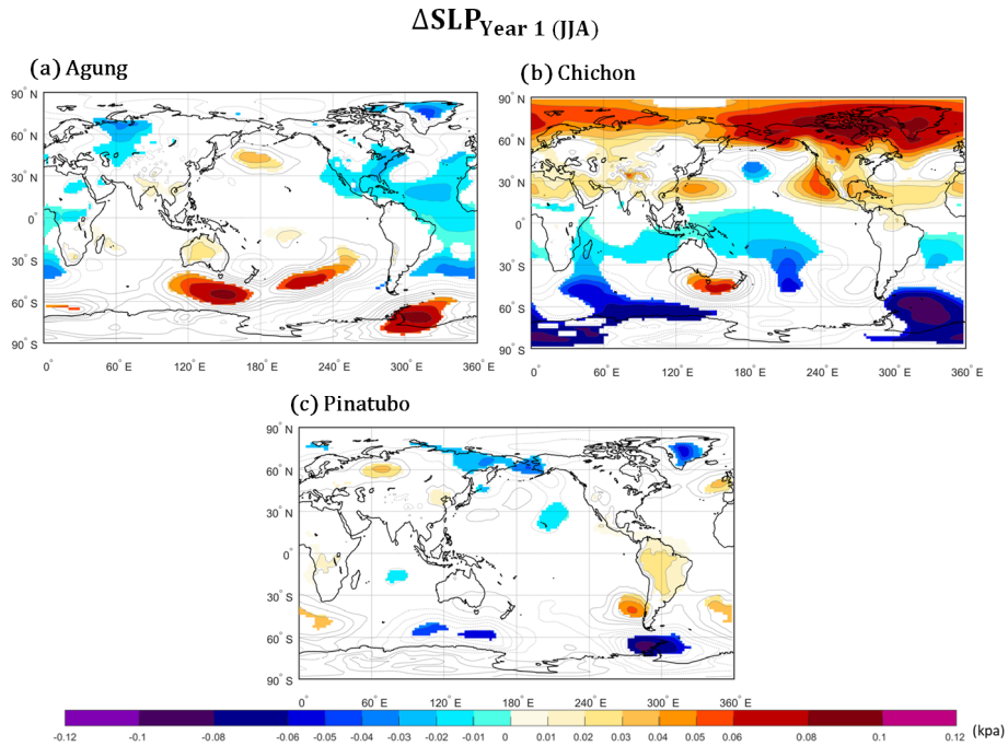
Figure A10. Ensemble average of change in the sea level pressure between the climatology and the volcano case for the first summer after the Agung (a), El Chichón (b) and Pinatubo (c) eruptions. Only significant anomalies are shown with an approximate 95 % confidence level using Student’s t test. Contours show SLP anomalies following the colour bar scale (solid line for positive anomalies and dashed line for negative anomalies).
