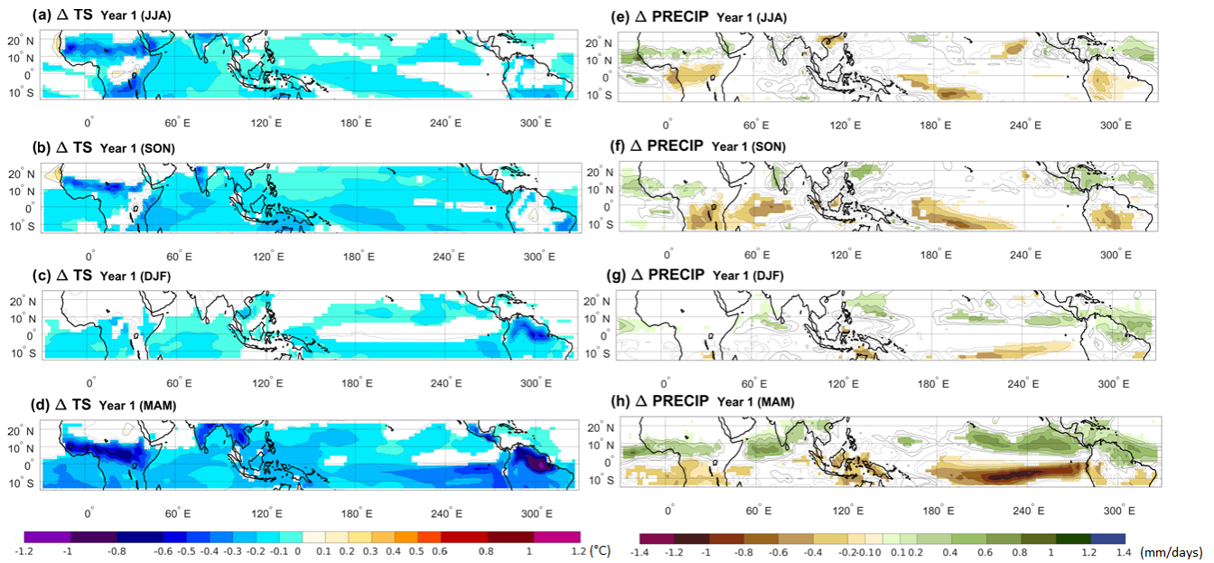
Figure A3. Ensemble mean of changes in surface temperature (a, b, c, d) and precipitation (e, f, g, h) between the climatology and the volcano case for each season of the year after the Agung eruption. Only significant anomalies are shown with an approximate 95 % confidence level using Student’s t test. Contours show temperature and precipitation anomalies following the colour bar scale (solid line for positive anomalies and dashed line for negative anomalies).
