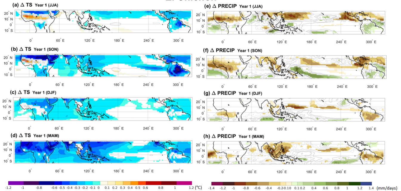
Figure A4. Ensemble mean of changes in surface temperature (a, b, c, d) and precipitation (e, f, g, h) between the climatology and the volcano case for each season of the year after the El Chichón eruption. Only significant anomalies are shown with an approximate 95 % confidence level using Student’s t test. Contours show temperature and precipitation anomalies following the colour bar scale (solid line for positive anomalies and dashed line for negative anomalies).
