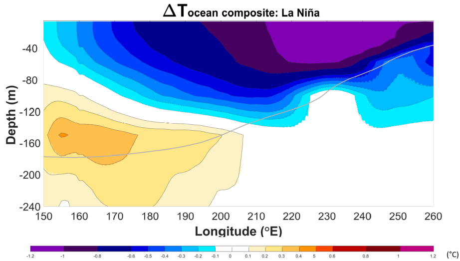
Figure A17. Temperature composite of La Niña events (Niño3.4 index \leq 0.4 °C) for a transect in the equatorial Pacific (averaged between 5° S and 5° N) in the reference period of each eruption (4 years before each eruption) and for the winter season (DJF). A total of 100 ensemble members are considered, leading to a total of 1200 years as a reference period and 237 La Niña events. Contours show the SST anomalies following the colour bar scale (solid lines for positive anomalies and dashed lines for negative anomalies; the 0 line is omitted). The bold grey line shows the climatological thermocline depth (as defined using the 20 °C isotherm).
