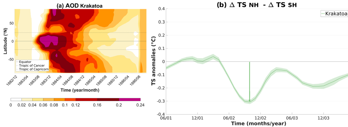
Figure A6. Evolution of the aerosol optical depth and ensemble average of the difference between the cooling of the SH ( \Delta T \text{ SH} ) and the NH ( \Delta T \text{ NH} ) for the Krakatau eruption. (a) The band of wavelength used is between approximately 462 and 625 nm. (b) The 3-year climatology is subtracted to calculate the anomalies. Shading represents twice the standard error of the ensemble mean (i.e. \sim 95\% confidence interval).
