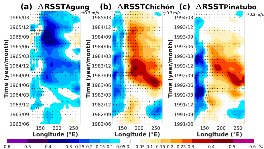
Figure 3. Hovmöller plot of the ensemble mean of the relative SST anomalies in the equatorial Pacific (averaged over -5 and 5^{\circ} N) and the change in the zonal component of the 10 m winds (m/s) for the 3 years following each eruption. The anomalies are calculated relative to the 3 years before each eruption.
