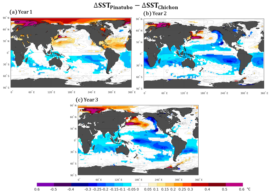
Figure A9. Difference in the ensemble mean sea surface temperature anomalies between the Pinatubo and El Chichón eruptions ( \Delta TS_{\text{Pinatubo}} - \Delta TS_{\text{Chichón}} ). Only significant anomalies are shown with an approximate 95 % confidence level using Student’s t test. Contours show temperature anomalies following the colour bar scale (solid line for positive anomalies and dashed line for negative anomalies).
