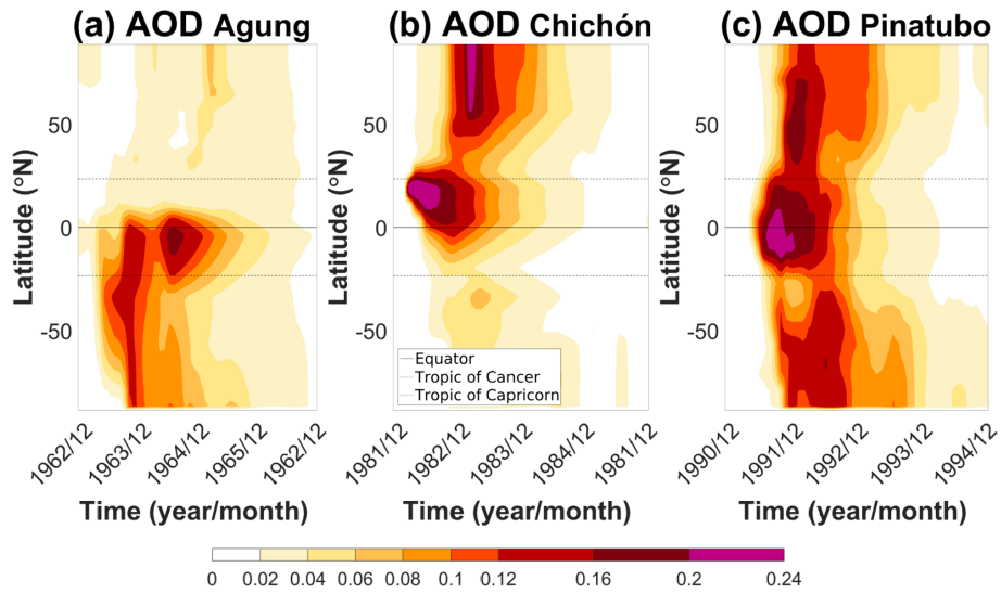
Figure 1. Evolution of the aerosol optical depth during 4 years for the three eruptions. The band of wavelength used is between approximately 462 and 625 nm.
