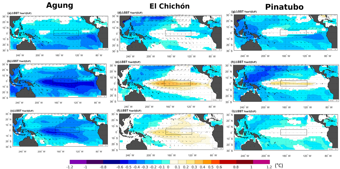
Figure A11. Ensemble mean of changes in sea surface temperature (SST) (shadings) and 10 m winds (arrows) between the volcano case and the climatology for each of the following three winter seasons (DJF) after the Agung (a–c), El Chichón (d–f) and Pinatubo (g–i) eruptions. Only significant SST changes are shaded with an approximate 95 % confidence level using Student’s t test. Contours show the SST anomalies following the colour bar scale (solid lines for positive anomalies and dashed lines for negative anomalies; the 0 line is omitted). The boxes indicate the Niño 3.4 area.
