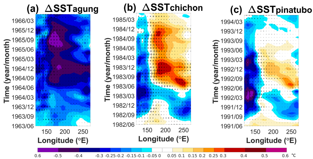
Figure A12. Hovmöller plot of the ensemble mean of the SST anomalies in the equatorial Pacific (averaged over -5 and 5^{\circ} N) and the change in the zonal component of the 10 m winds (m/s) for the 3 years following each eruption. The anomalies are calculated relative to the 3 years before each eruption.
