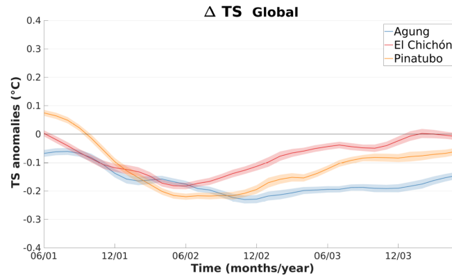
Figure A1. Evolution of the ensemble mean of the global cooling in the three eruption cases for 3 years, starting at the first summer after the eruption. The 3-year climatology is subtracted to calculate the anomalies. Shading represents twice the standard error of the ensemble mean (i.e. \sim 95\% confidence interval).
