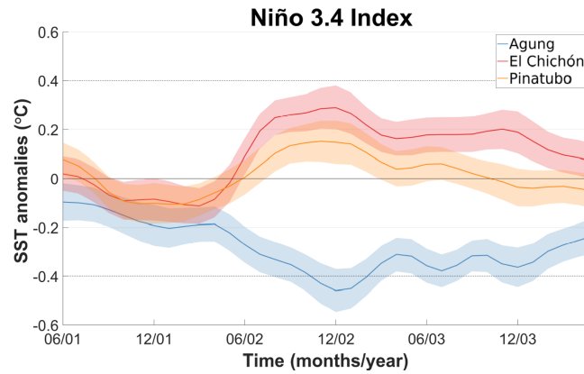
Figure A13. Ensemble mean changes in the Niño 3.4 index after each eruption. The 3-year climatology is subtracted to calculate the anomalies. Shading represents twice the standard error of the mean using an approximate 95 % confidence interval.
