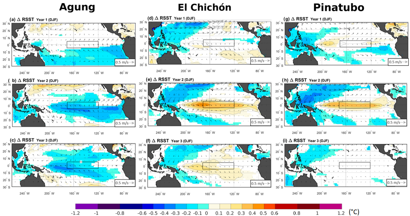
Figure 2. Ensemble mean of changes in relative sea surface temperature (RSST) (shadings) and 10 m winds (arrows) between the volcano case and the climatology for each of the following three winter seasons (DJF) after the Agung (a–c), El Chichón (d–f), and Pinatubo (g–i) eruptions. Only significant RSST changes are shaded with an approximate 95 % confidence level using Student’s t test. Contours show the RSST anomalies following the colour bar scale (solid lines for positive anomalies and dashed lines for negative anomalies; the 0 line is omitted). The boxes indicate the Niño 3.4 area.
