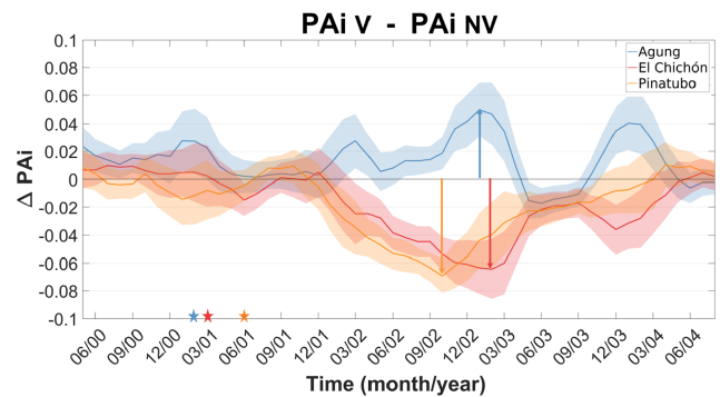
Figure 7. Evolution of the difference in the ensemble mean between the precipitation asymmetry index (PAi V ) and the climatology (PAi NV ). Shading represents twice the standard error of the ensemble mean (i.e. ~ 95 % confidence interval). The three stars represents the moment of each eruption.
