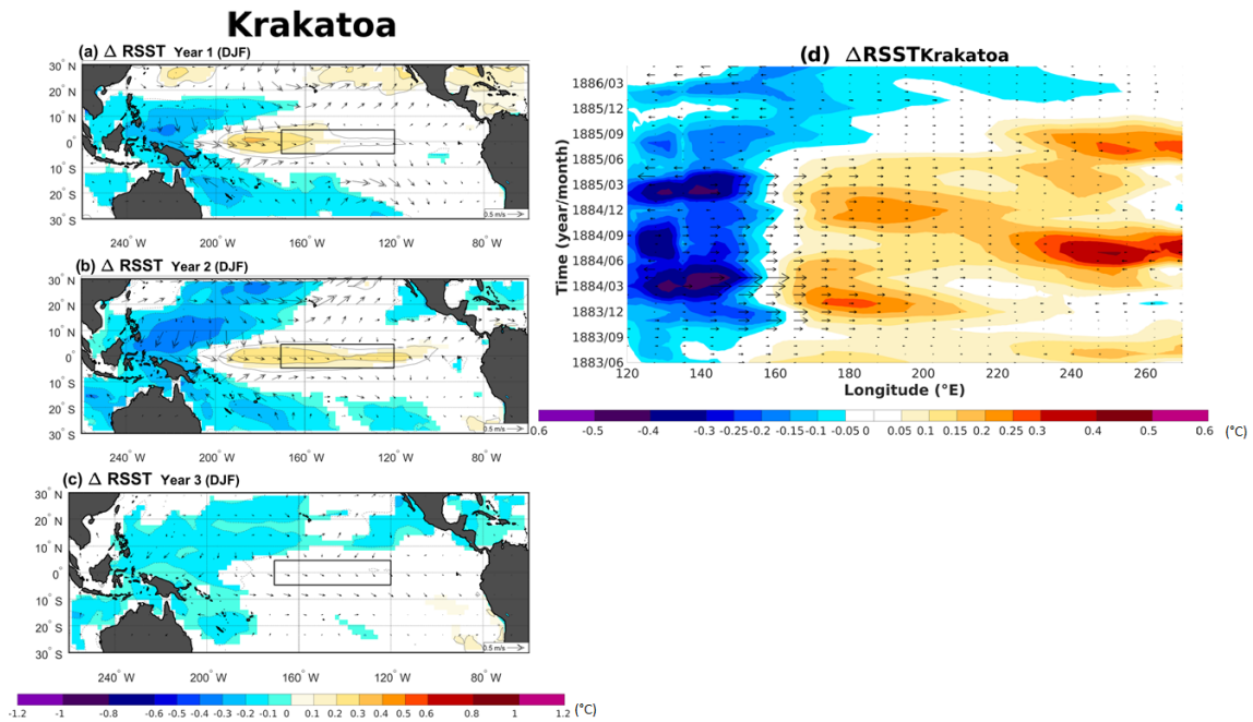
Figure A7. Ensemble mean of changes in relative sea surface temperature anomalies and 10 m winds (arrows) between the climatology and the volcano case for the three winter seasons (DJF) after the Krakatau eruption. Only significant RSST changes are shown with an approximate 95 % confidence level using Student’s t test. Contours show the RSST anomalies following the colour bar scale (solid lines for positive anomalies and dashed lines for negative anomalies). The boxes indicate the Niño 3.4 area.
