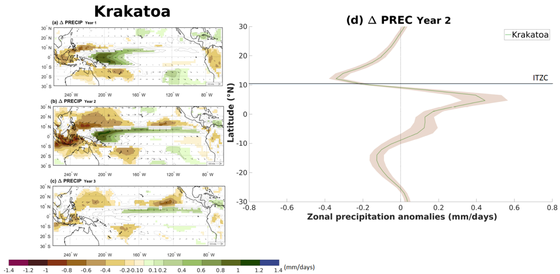
Figure A8. (a, b, c) Ensemble mean of changes in precipitation and 10 m wind (arrows) between the 3-year climatology and the volcano case for the three summer-to-winter seasons (June to February) following the Krakatau eruption. Only precipitation changes that are significant at the 95 % confidence level using Student’s t test are shaded. Contours show the precipitation anomaly following the colour bar scale (solid lines for positive anomalies and dashed lines for negative anomalies; the 0 line is omitted). (d) Ensemble average of the zonal precipitation anomaly over the Pacific Ocean (160° E–100° W) between the 3-year climatology and the summer-to-winter season (June to February) of the second year after the Krakatau eruption. Shading represents twice the standard error of the ensemble mean (i.e. ~95 % confidence interval). The blue line highlights the ensemble-averaged 3-year climatology position of the ITCZ (defined as the location of the zonal-average precipitation maximum).
