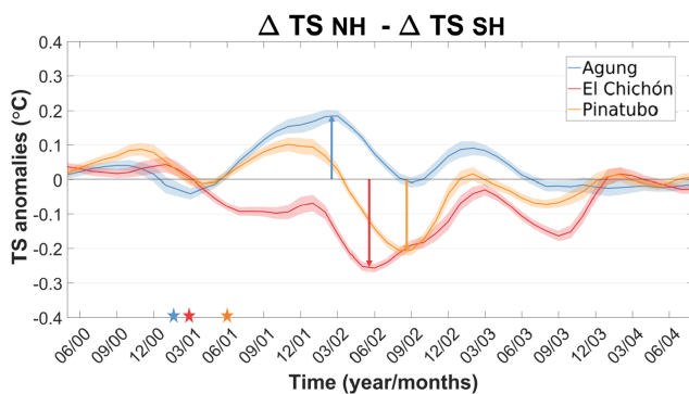
Figure 4. Evolution of the difference in the ensemble mean between the volcanically induced cooling of the SH and the NH after each eruption ( \Delta T_{\text{NH}} - \Delta T_{\text{SH}} ). Shading represents twice the standard error of the ensemble mean (i.e. \sim 95\% confidence interval).
