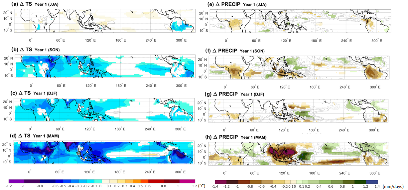
Figure A5. Ensemble mean of changes in surface temperature (a, b, c, d) and precipitation (e, f, g, h) between the climatology and the volcano case for each season of the year after the Pinatubo eruption. Only significant anomalies are shown with an approximate 95% confidence level using Student’s t test. Contours show temperature and precipitation anomalies following the colour bar scale (solid line for positive anomalies and dashed line for negative anomalies).
