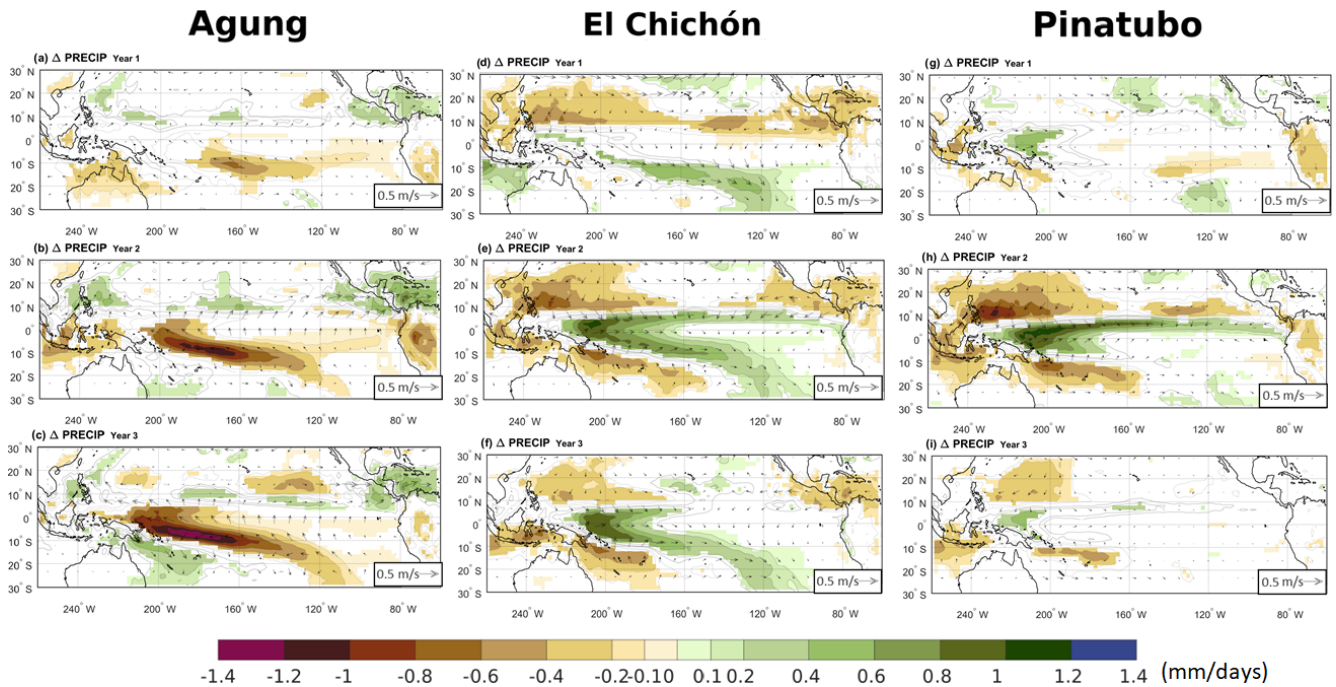
Figure 5. Change in ensemble mean precipitation and 10 m winds (arrows) between the reference years and the volcano case for the three summer to winter seasons (June to February) following the Agung (a–c), El Chichón (d–f) and Pinatubo (g–i) eruptions. Contours show the precipitation anomaly following the colour bar scale (solid lines for positive anomalies and dashed lines for negative anomalies, the 0 line is omitted). Only precipitation changes that are significant at the 95 % confidence level using Student’s t test are shaded.
