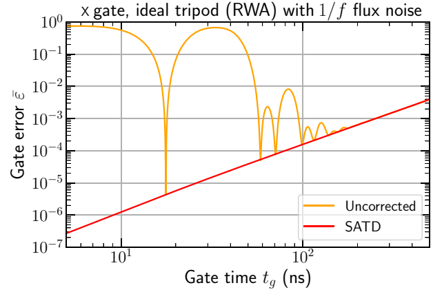
FIG. 9. State-averaged gate error \bar{\varepsilon} = 1 - \bar{F} as a function of gate time t_g for ideal (four-level, RWA) tripod X gates. We compare uncorrected adiabatic pulses (orange curve) against the accelerated SATD pulses (red curve) in the presence of 1/f flux noise. The scale of the uncorrected pulses is set by \Omega_0/2\pi = 100 MHz, and the 1/f flux noise has a strength parameterized by A_{\Phi_{\text{ext}}} = 3\mu\Phi_0 (yielding a qubit dephasing time T_{\varphi,01} = 7 \mu\text{s} ). Fluxonium parameters match those given in the caption for Fig. 6.
