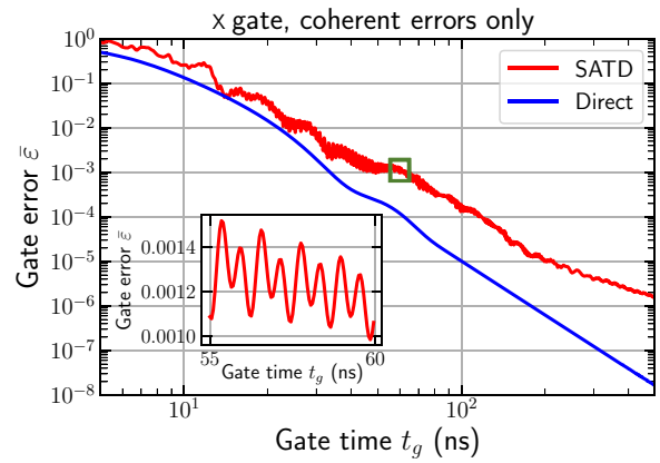
FIG. 10. State-averaged gate error \bar{\epsilon} = 1 - \bar{F} as a function of gate time t_g , for SATD tripod (red curve) and direct-driving (blue curve) realizations of a fluxonium X gate. Dissipation is not included here, but non-RWA error channels are. The inset shows an enlargement of the SATD gate error. The gates are calculated with the 18 lowest energy levels of the circuit. For the SATD gate, we use the optimal uncorrected gap frequency \Omega_0/2\pi = 1.135/t_g that minimizes the rms voltage at each gate time t_g . The fluxonium parameters are as for Fig. 6.
