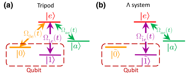
FIG. 2. (a) An ideal tripod system consisting of three lower energy levels (the qubit states |0\rangle and |1\rangle ) as well as the auxiliary state |a\rangle ) resonantly coupled to an excited state |e\rangle by three different driving tones, with envelopes \Omega_{0e}(t) , \Omega_{1e}(t) , and \Omega_{ae}(t) , respectively. (b) An effective \Lambda system (consisting of the state |\tilde{1}\rangle and the state |a\rangle resonantly coupled to the state |e\rangle ) used to describe the dynamics of the tripod system. The control pulses \Omega_{\tilde{1}e}(t) and \Omega_{ae}(t) perform a double STIRAP protocol that cyclically evolves the zero-energy dark states in the \Lambda system.
