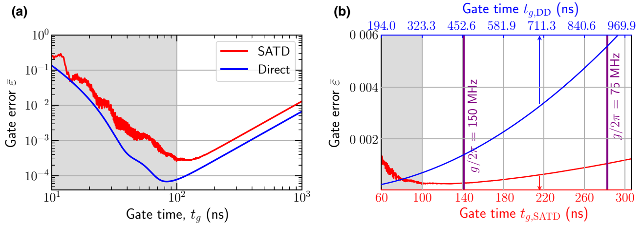
FIG. 11. Comparison between state-averaged X-gate error \bar{\epsilon} = 1 - \bar{F} for SATD (red curve) and direct-driving (blue curve) protocols in our fluxonium system, including effects of 1/f flux noise dephasing as well as non-RWA errors; 18 fluxonium levels are included in the simulations. Dephasing is treated as per Sec. VI B1 with a 1/f flux noise amplitude A_{\Phi_{\text{ext}}} = 3\mu\Phi_0 corresponding to the qubit dephasing time T_{\varphi,01} = 7 \mu\text{s} . (a) Log-log plot of gate error \bar{\epsilon} versus gate time t_g . For each time, the DD protocol has a smaller error but uses significantly larger pulse amplitudes. (b) Linear plot of gate error \bar{\epsilon} for both protocols at equal power levels \bar{V}_{\text{rms}} [see Eq. (30)]. The shaded (unshaded) region corresponds to the time regime where the gate errors are dominated by non-RWA errors (dephasing). For the same value of \bar{V}_{\text{rms}} , the gate time for the DD protocol is longer than for the SATD protocol (hence the two distinct x axes). Vertical lines indicate the shortest gate times possible [corresponding to the maximum allowed \bar{V}_{\text{rms}} ; see Eq. (32)] for cavity-based driving for time-averaged cavity photon number \bar{n}_{\text{cav}} = 0.05 and a fixed cavity-fluxonium coupling g (purple vertical lines). Fluxonium parameters are the same as for Fig. 6.
