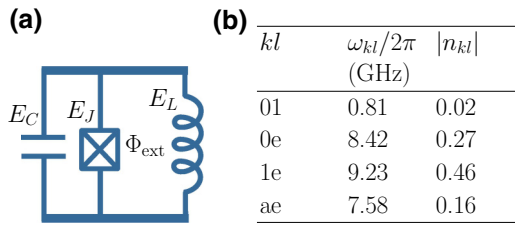
FIG. 6. (a) Circuit diagram of a fluxonium. (b) The qubit and tripod transition frequencies ( \omega_{kl} ) as well as the magnitude of the charge matrix elements ( n_{kl} ) of the fluxonium whose energy spectrum is given in Fig. 1. The computational states in the tripod system are labeled by |0\rangle , |1\rangle , |a\rangle , and |e\rangle . The fluxonium parameters used to get the values of \omega_{kl} and n_{kl} in (b) are E_L/h = 0.063 GHz, E_J/h = 9.19 GHz, E_C/h = 2 GHz, and \Phi_{\text{ext}} = 0.17\Phi_0 .
