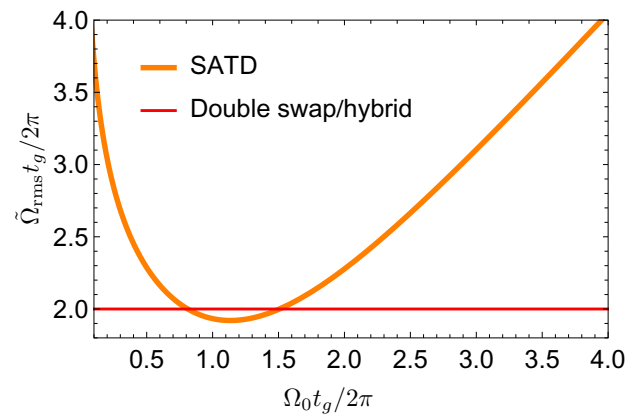
FIG. 5. \tilde{\Omega}_{\text{rms}} t_g / 2\pi versus \Omega_0 t_g / 2\pi for the SATD protocol (orange curve) as well as the double swap protocol and the hybrid protocol (red line). For the SATD protocol, \tilde{\Omega}_{\text{rms}} = \Omega_0 in the adiabatic limit ( \Omega_0 t_g \rightarrow \infty ). Away from the adiabatic limit, the SATD correction increases \tilde{\Omega}_{\text{rms}} above \Omega_0 . The minimum of the SATD plot is \tilde{\Omega}_{\text{rms}} t_g / 2\pi = 1.92 , occurring at \Omega_0 t_g / 2\pi = 1.135 . The red line \tilde{\Omega}_{\text{rms}} t_g / 2\pi = 2 is the value of \tilde{\Omega}_{\text{rms}} for the double-swap protocol and the hybrid protocol.
