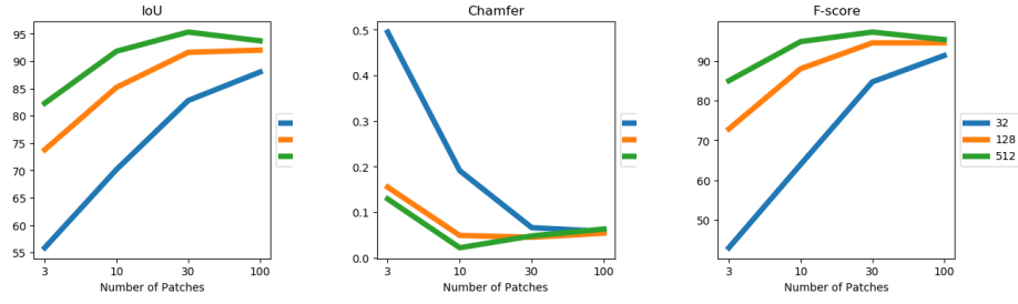
Fig. S.3. Mean error metrics on the reduced ShapeNet test set for different numbers of patches and network/latent code sizes.
