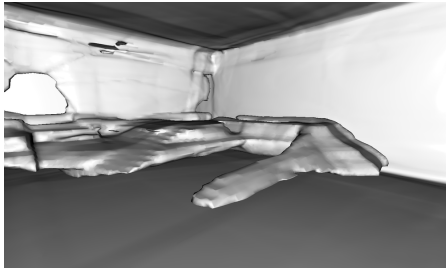
DeepSDF
