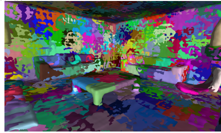
Patches (Ours)
