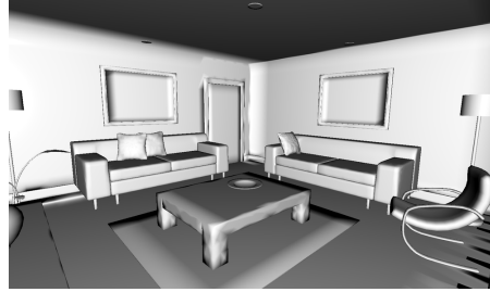
Groundtruth
