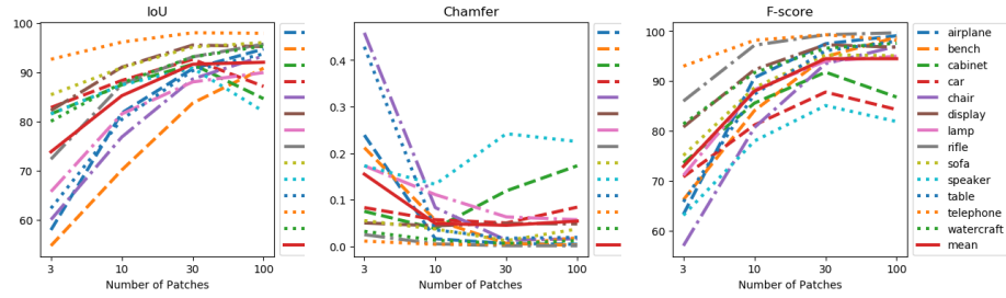
Fig. S.4. Per-category error metrics on the reduced ShapeNet test set for different numbers of patches.
