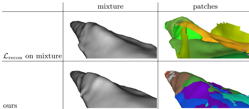
Fig. S.1. Mixture Reconstruction Loss. Imposing the reconstruction loss on the mixture instead of directly on the patches leads to individual patches not matching the surface.
