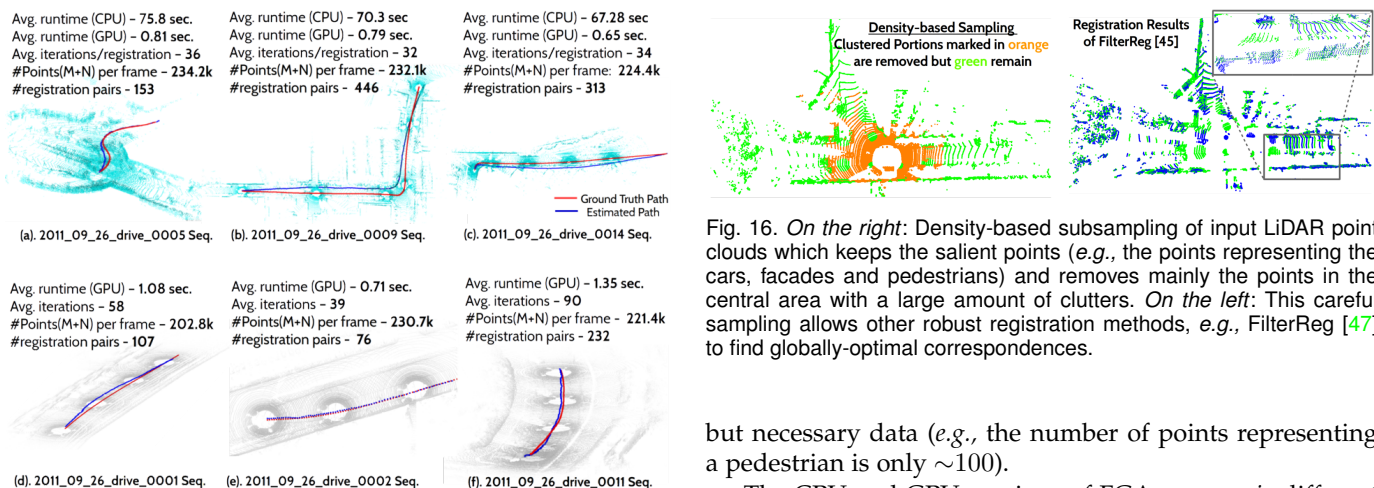
Fig. 15. Consecutive frame-wise registrations of LiDAR point clouds from six different driving sequences of the KITTI-RAW [94] dataset by our FGA. The ground-truth paths are compared with the estimated paths, which reflects minimum drift and transformation error. In the first row, the driving sequences have more turns in the trajectories of sensor-carrying vehicle. In contrast, the vehicle trajectories in the second row have relatively more pronounced rectilinear motion than in the first row.
