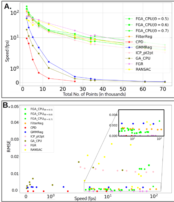
Fig. 6. (A:) Throughput of different methods in frames per second and (B:) Bivariate correlation plot for the alignment accuracy and speed, for ten data sizes and random initial misalignments. The bottom right area of the plot, dominated by FGA, reflects the most efficient marks.
