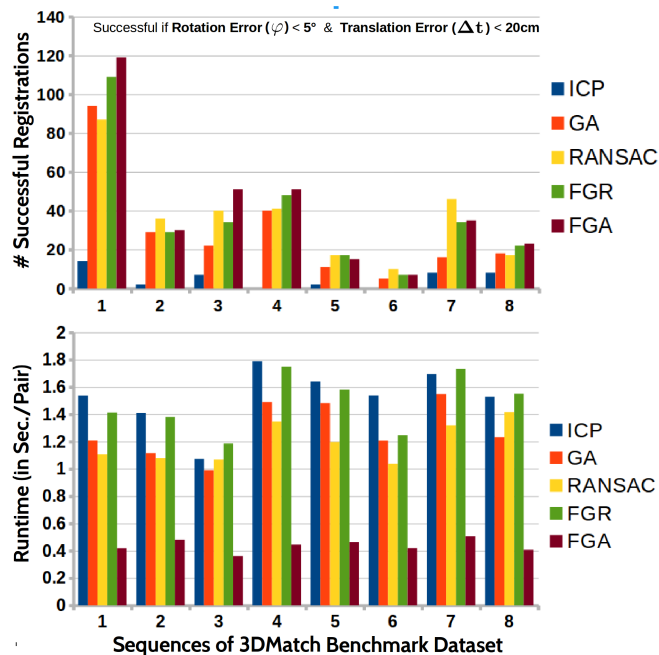
Fig. 10. Our FGA is tested on eight evaluation sets of 3DMatch [67] dataset. We define a strict measurement ( i.e. , when the angular error is less than 5^\circ and translational error is less than 20 centimeters) to count successful registrations. Top plot : The success rate of FGA is compared against the previously well-performing methods — FGR [20], RANSAC [19] and two other baseline methods — GA [10] and ICP [6]. Bottom plot : FGA records the fastest runtime of \sim 0.423 seconds, including mass computation via SPM function, on average per a scan pair.
