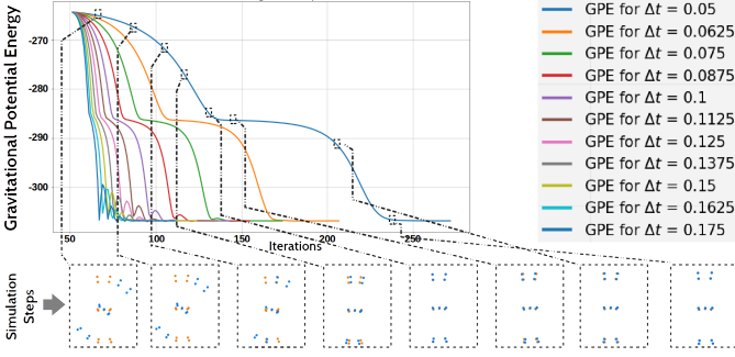
Fig. 2. GPE function plot with different optimization momenta handled by the increasing time differential (time step \Delta t ). Simulation steps depict the reference-template configuration at the current iteration.
