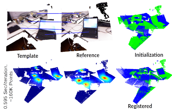
Fig. 11. FGA applied on template and reference point clouds (frames 1 and 10 from Freiburg [27] dataset). Top row : input images with the prior correspondences and the initialization on the right. Bottom row : Our SPM (S) function radially distributes weights around four different prior landmarks (highlighted by blue lines), and the alignment on the right.
