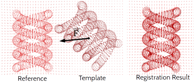
Fig. 1. Fast Gravitational Approach for rigid point set registration: template is attracted by the gravitational forces \mathbf{F} induced by the reference . The velocity and positions of template points are individually updated by solving equations of particle motion in a viscous medium, whereupon rigidity constraints are applied. Left: initial misalignment of the helix [22]; Right: registration result after 150 iterations (without acceleration and boundary conditions) by GA [10] or 48 iterations (using the acceleration technique and boundary conditions) by FGA (our improved method).
