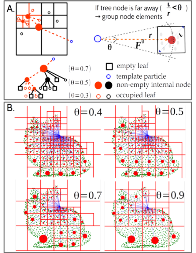
Fig. 3. (A): BH tree structure with hierarchical cell grouping and pruning depends on the node opening criteria \theta . (B): BH force approximation \mathbf{F}^\theta [23] under different values of the node opening parameter \theta for a template point set (in green color). The red dots represent the CoM of the cells with sizes proportional to the number of points inside the nodes.
