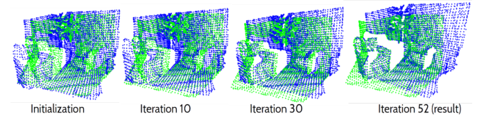
Fig. 8. A sample result of FGA tested with two frames (separated by four consecutive frames) with moderate partial overlaps from the Stanford lounge dataset [98].
