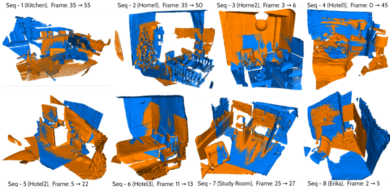
Fig. 9. Sample pairwise registration results of our method on all eight different test scenes in 3DMatch [67] dataset. The input point set pairs exhibit minimal overlaps and irregular cropped areas. The template \mathcal{Y} is colored blue and the reference is colored orange. Results of FGA named by the source-to-target frames ( i \rightarrow j ) are best viewed in color.
