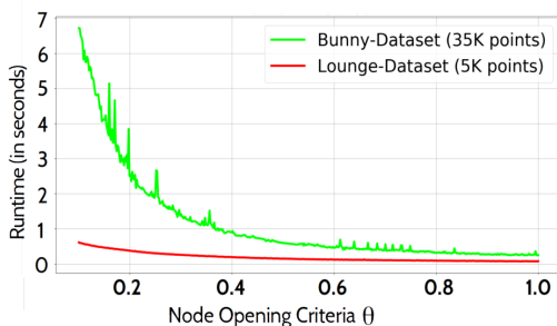
Fig. 7. Runtime (in seconds) of FGA for increasing values of the node opening criteria \theta in FGA.
