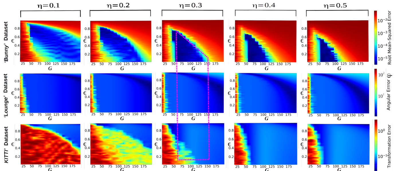
Fig. 18. Selecting best FGA parameters with a grid search method on G , \epsilon and \eta (slices for \eta = 0.1, 0.2, 0.3, 0.4 and 0.5 ). These parameters can be set from the common and wide area (value ranges) marked by the polygon in the middle. The parameter settings for our experiments are drawn from this region. Another figure like this would also draw the same conclusion on datasets scaled within other ranges (e.g., [-1, 1] ).
