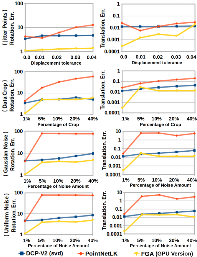
Fig. 5. The accuracy of our FGA and two deep learning methods PointNetLK [60] and DCP [61] trained on ModelNet40 [97] dataset, with additional 10% of the samples included in the training set after applying four different types of data disturbances. Our FGA is compared on five different validation sets with increasing levels of data disturbances. The error plots show that FGA outperforms the other two methods and highlight the robustness issues of the learning-based approaches.
