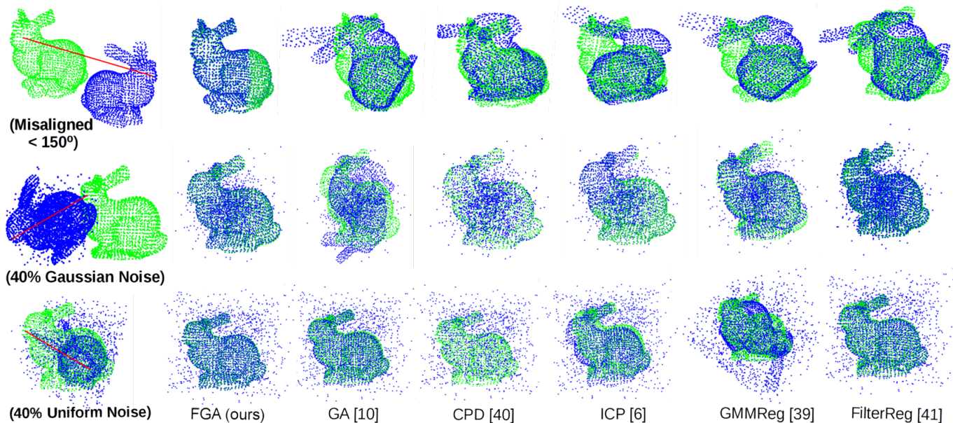
Fig. 13. Exemplary registration results in the experiment with the data disturbances (applying large misalignment, 40% of Gaussian noise, and 40% of uniformly distributed noise on the template Y ). Our FGA uses one prior match in this visualization and outperforms competing methods also without prior correspondences. See Table 2 for complete quantitative results (also without prior correspondences).
