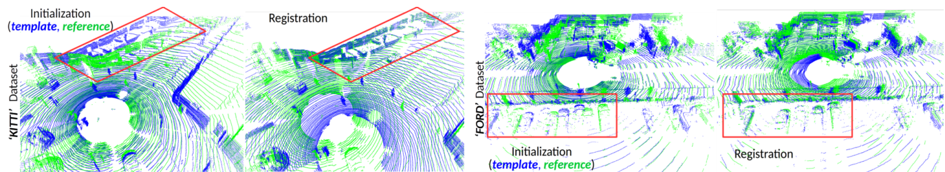
Fig. 14. Registration results of FGA on KITTI [94] and Ford Campus Vision [99] datasets without subsampling. Left : frames 1 and 20 as Y and X , respectively ( M + N \approx 245k points) from 2011_09_26_drive_0005_sync driving sequence. Right : frames 1000 and 1010 as Y and X ( M + N \approx 150K points). In both cases, no landmarks are available.
