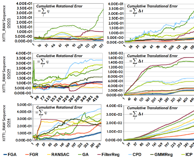
Fig. 17. Quantitative evaluation of several methods on the KITTI-RAW dataset. Plots show cumulative rotational and translational errors accumulated over pairwise registrations of all consecutive frames. Cumulative translational errors remain lowest across the frames for a given sequence in the case of our FGA. Only FGR [20] and RANSAC [19] show either comparable or higher accuracy over a few short subsequences.
