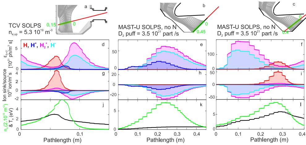
Figure 10. Profiles along an indicated line of sight of the various emission processes, particle source/sink processes as well as the electron temperature and density. This is shown for one TCX case and for two different line of sights for the same MAST-U case. The used line of sights, as well as the divertor geometry and the region where the lines of sight intersect the SOLPS grids are shown.
