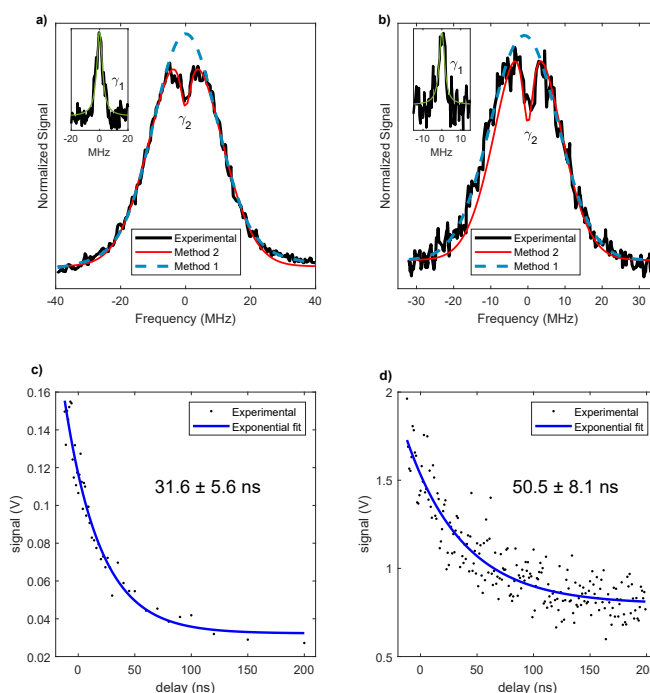
Fig. 6 Lifetime measurements of the S_1 excited state. a) and b) show Lamb dip measurement of eq1 and ax2 , respectively. The experimental data is plotted in black, the blue curve is the fit to a Voigt profile. The subtraction of these two curves is shown in the inset, together with its fit to a Lorentzian (green curve). The red curve is the fit using the saturated absorption coefficient which determines D_0 and \gamma_s . c) and d) are the two-color REMPI delay scans of eq1 and ax2 , respectively. The lifetimes are extracted by fitting the experimental measurements to two single exponential decays.
