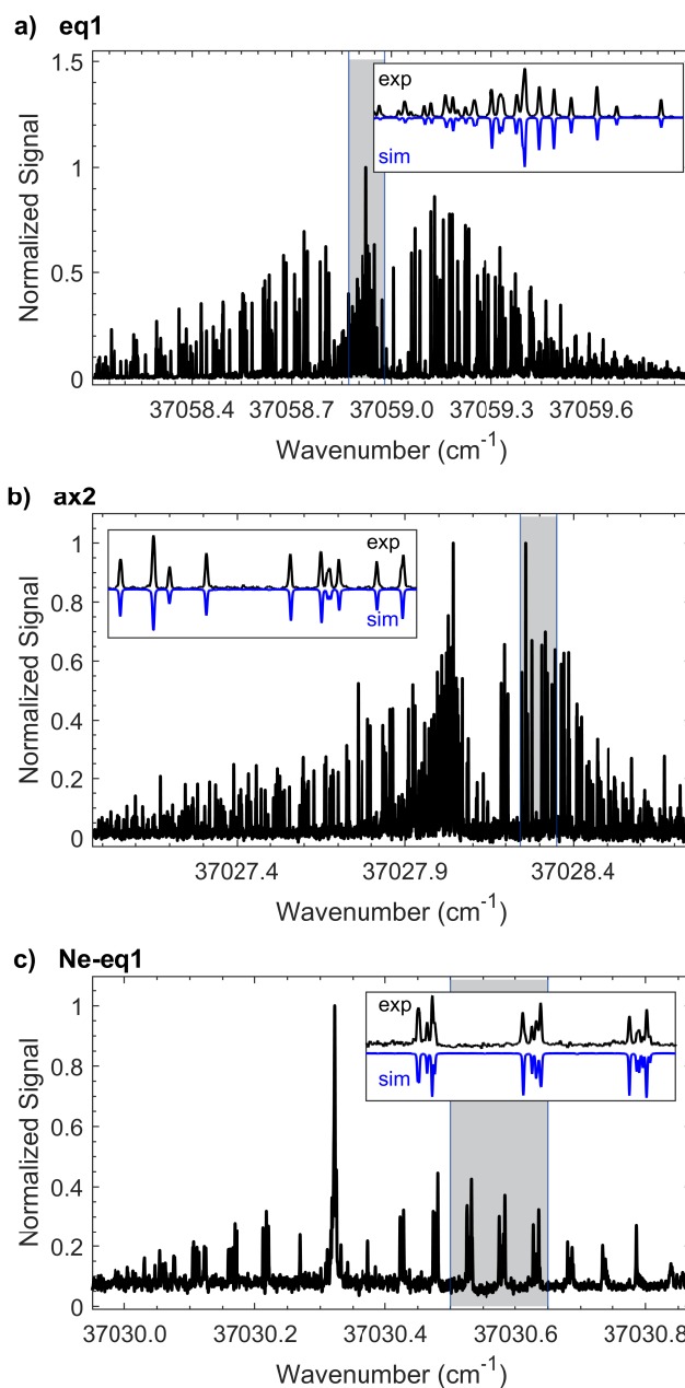
Fig. 4 HR-LIF spectra of 3 species of 1-indanol: a) Conformer eq1 recorded at \sim 1 K, b) Conformer ax2 recorded at \sim 1.5 K, and c) Neon complex Ne-eq1 recorded at \sim 1.5 K. In the insets the blue traces show the simulated spectra and the black traces are experimental data. These insets correspond to the domains shadowed with grey. These spectra were recorded at a scan rate of \sim 5 MHz per second.
