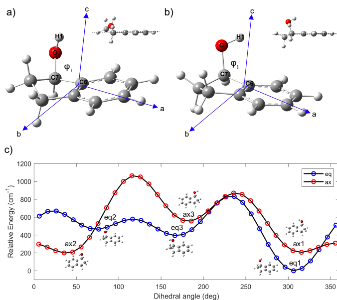
Fig. 1 Conformational landscape of 1-Indanol. a) Lowest energy conformer eq1, with inertial axes as indicated. The inset visualizes the equatorial position of the OH group with respect to the 5-membered ring. b) Second-lowest energy conformer ax2 with inertial axes as indicated. The inset visualizes the axial position of the OH group with respect to the 5-membered ring. c) Cut of the calculated potential energy surface along the the dihedral angle, \phi_1 , for the equatorial and axial configurations.
