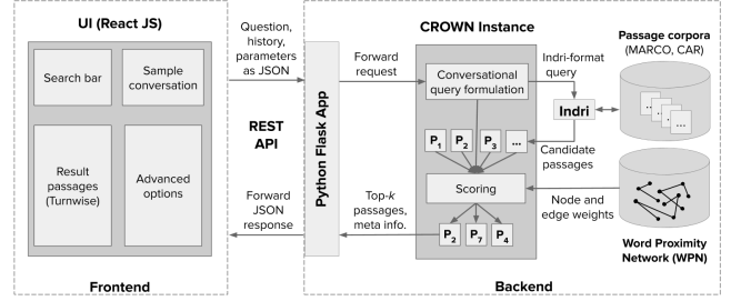
Figure 2: Overview of the CROWN architecture.
