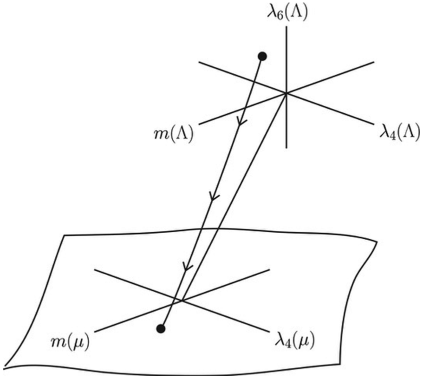
Figure 1. Renormalization group flow of scalar field theories to a surface spanned by renormalizable parameters.
