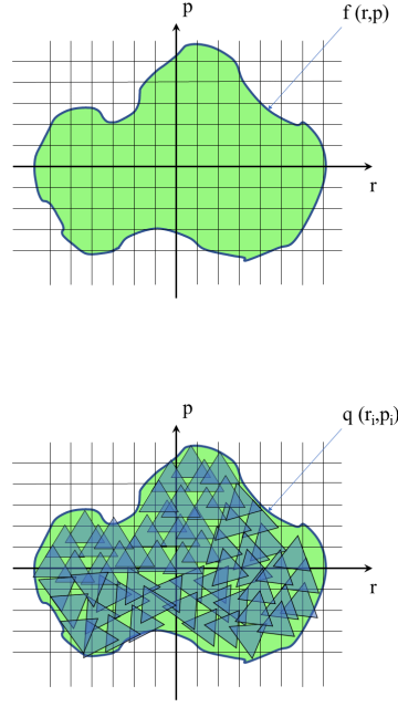
Figure 2.1: :Figure showing the relation between Vlasov (top) and PIC (bottom) codes. The figure is adapted from [156].
