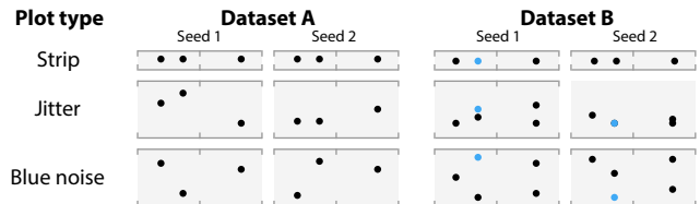
Figure 2: Three different plotting approaches (rows) for two different univariate datasets at two different random seeds (columns). Strip plots always fail to convey the datasets, as they look the same. Jitter plots, may sometimes fail: dataset B looks like dataset A for seed 2 while they are different. Our Blue Noise Plot never fails.
