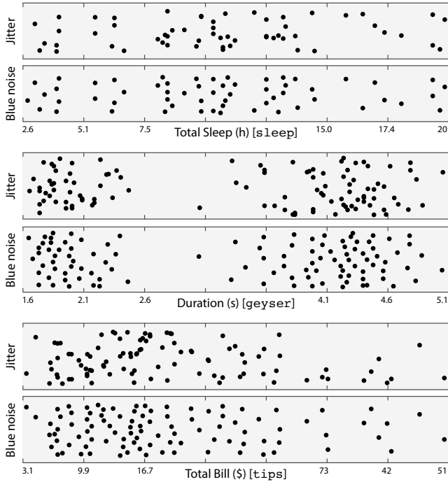
Figure 6: Comparison of three different data sets, each of them visualized using a traditional jitter plot and our Blue Noise Plot.
