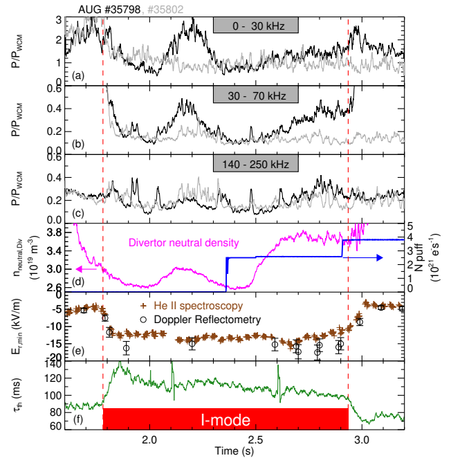
FIG. 8: Density fluctuation power in different frequency bands (a – c) reacting to N seeding (d). Divertor neutral density (d) and edge radial electric field minimum (e) are also displayed. The energy confinement time (f) decreases as N is added to the discharge (cf Fig. 1). For reference, fluctuation powers from a non-seeded comparison discharge are shown (grey, a – c).
