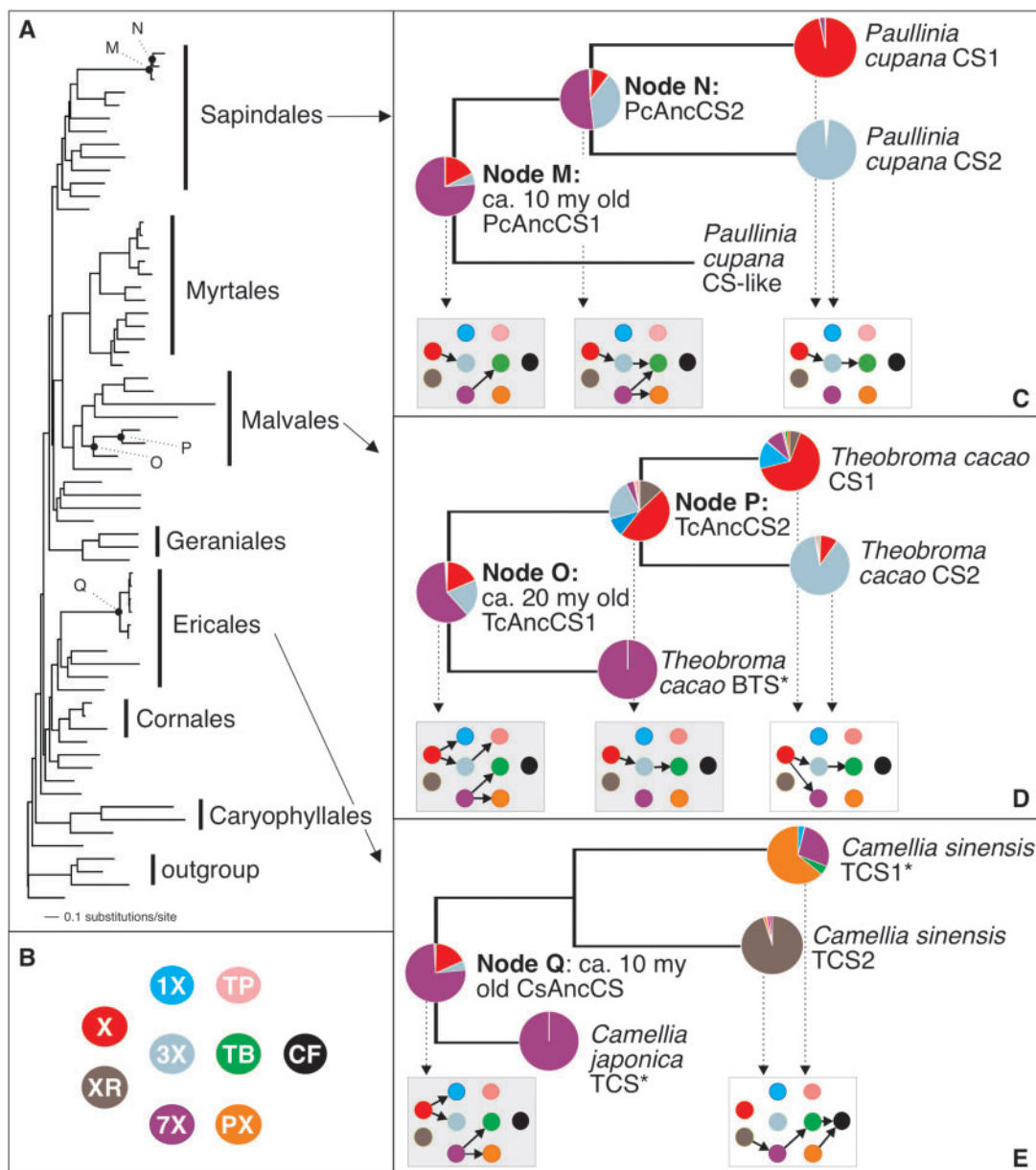
Fig. 2. Substrate preferences of ancestral CS-type enzymes reveal the origins of modern-day enzyme activities. (A) Estimated CS gene tree (lnL = -19,220.31407) shows general relationships among sequences from divergent orders of angiosperms. Node labels are shown for reconstructed ancestral enzymes. (B) Xanthine alkaloid substrates tested with each CS enzyme are color-coded to represent structures shown in figure 1. X = xanthine, XR = xanthosine, 1X = 1-methylxanthine, 3X = 3-methylxanthine, 7X = 7-methylxanthine, TP = theophylline, TB = theobromine, PX = paraxanthine, CF = caffeine. (C) Ancestral Paullinia CS enzymes preferred to methylate 7X as shown by the pie charts at nodes M and N but ultimately evolved modern-day enzymes to sequentially methylate X and 3X and catalyze a complete pathway to TB. (D) Ancestral Theobroma CS enzyme at Node O preferred to methylate 7X. After duplication, preference for X evolved in the ancestral enzyme at Node P. From this enzyme, modern-day Theobroma CS enzymes evolved substrate preferences allowing for TB biosynthesis via sequential methylation of X and 3X. (E) Ancestral Camellia CS enzyme of Node Q also preferred to methylate 7X but later evolved divergent modern-day activities shown for C. sinensis TCS1 and TCS2. Inset boxes showing CF pathway network is shaded for ancestral enzymes. The pie charts of figure 2C–E represent mean relative activity with each substrate for the combined ancestral alleles at each node. Enzymes marked with “*” are taken from published studies from other laboratories.
