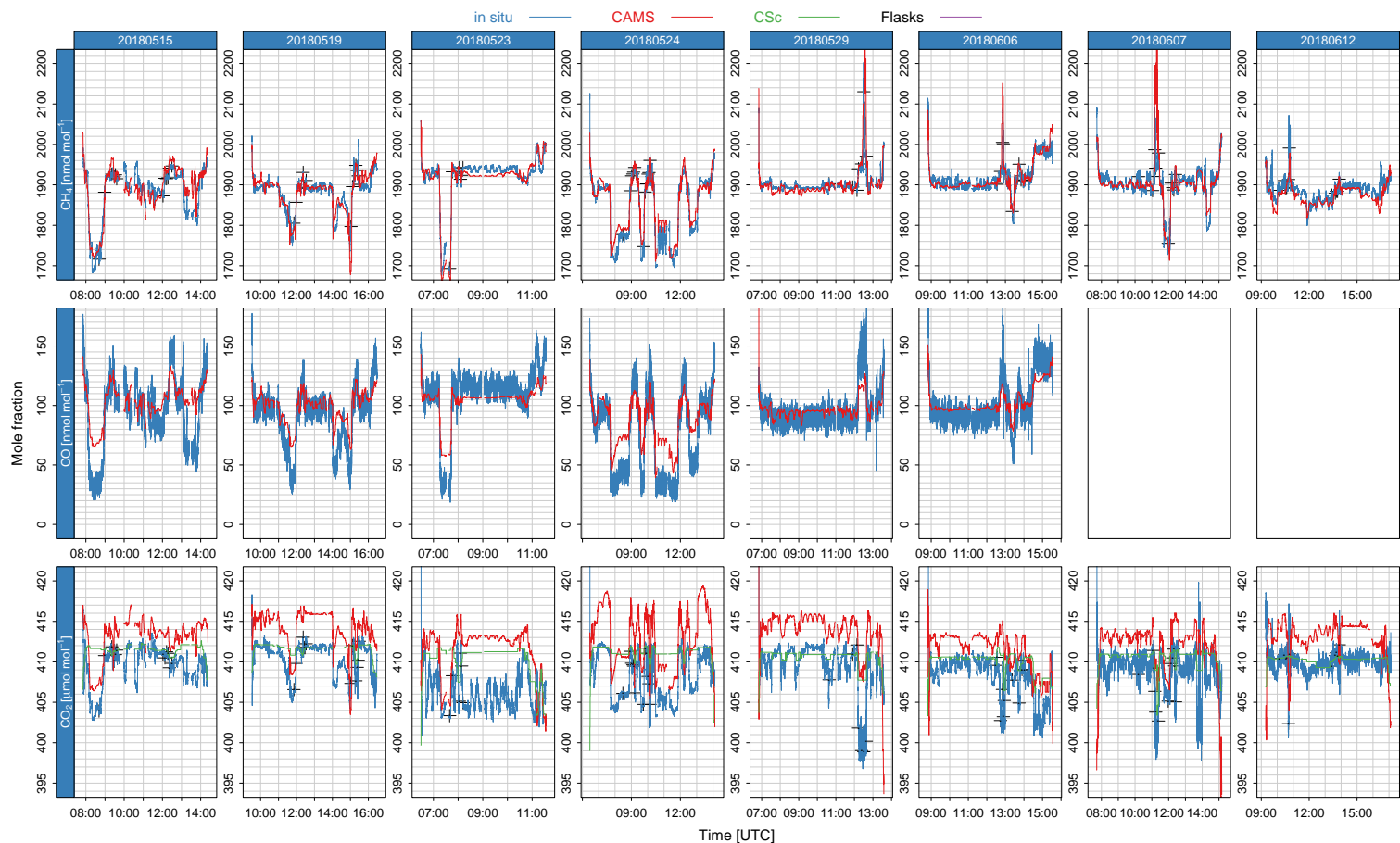
Figure S2. Time-plots of in situ measurements of CH 4 , CO and CO 2 performed throughout CoMet campaign aboard HALO aircraft with JIG instrument (blue). Model results from CAMS and CarboScope (denoted with CSc) extracted at respective time and aircraft coordinates are given in red and green, respectively. Results from flask samples collected with JAS marked with crosses. Shading denotes data flagged as "vertical profiles" and used for characterization of vertical structure of the atmosphere over the study area. Blue shading - ascending profile. Red shading - descending profile. CO data for flights on June 7 th and June 12 th discarded due to instrument malfunction. See the manuscript for details.
