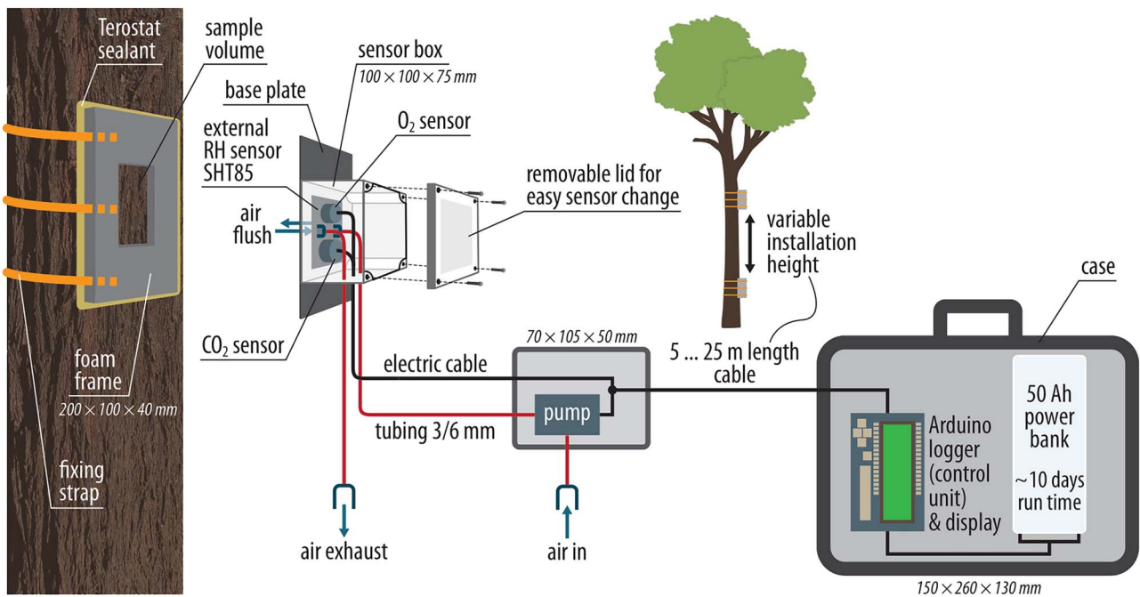
Figure 1. Custom-made modular stem gas exchange system featuring a \text{CO}_2 and an \text{O}_2 sensor for repeated cyclic measurements of changes in gas concentration over time within a closed dynamic stem chamber installed on the tree stem. A pump automatically flushes the chamber headspace between measurement cycles. The device is battery powered with up to 10 days operating time. An Arduino ® controls switching between measurement and flushing mode and logs the data on an SD card. ©Annett Börner
