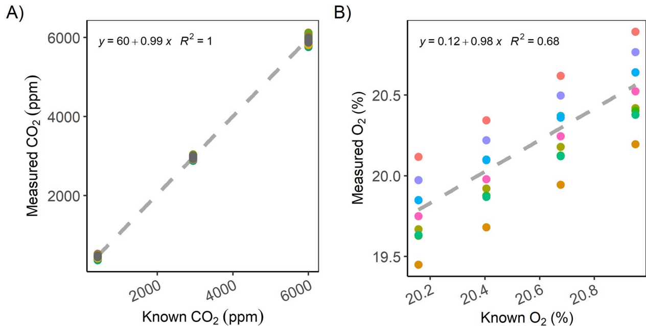
Figure 2. Measurements of known gas concentrations in the calibration and testing unit (25°C) for (A) CO 2 (CO 2 concentrations of 420, 2944 or 6020 p.p.m.) by COZIR sensors ( n = 10 ) and (B) O 2 (in %, dilution from 20.95 to 20.16%) by LuminOx sensors ( n = 10 ). Colours depict different sensor ID. The dashed line represents the linear regression.
