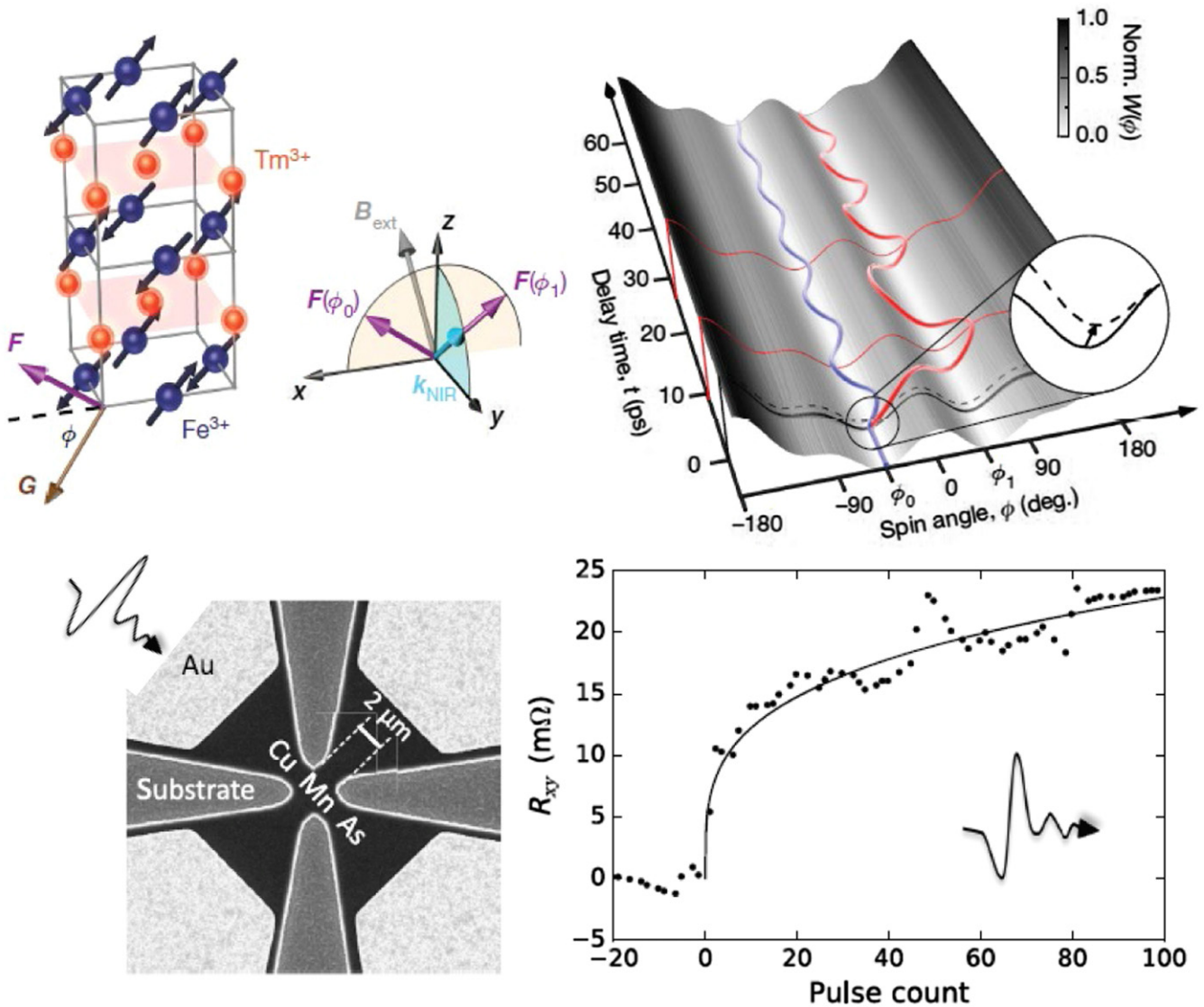
Figure 26. (a) Spin and lattice structure of TmFeO 3 . The ferromagnetic moment ( F ), antiferromagnetic vector ( G ), wave vector of the probe pulse ( k_{\text{NIR}} ), and external magnetic field ( B_{\text{ext}} ) are shown. On THz excitation, the magnetic potential W(\varphi) is abruptly modified. For a THz near field of E = 10 \text{ MV cm}^{-1} , the spins can be switched coherently by a single free space THz pulse (red trajectory) at \varphi_1 \sim \varphi_0 + 90^\circ . Reprinted by permission from Springer Nature Customer Service Centre GmbH: [Springer Nature] [Nature] [167] (2019). (b) CuMnAs device image. The multilevel memory signal as a function of the number of applied picosecond free space THz pulses. Reproduced from [168]. CC BY 4.0.
