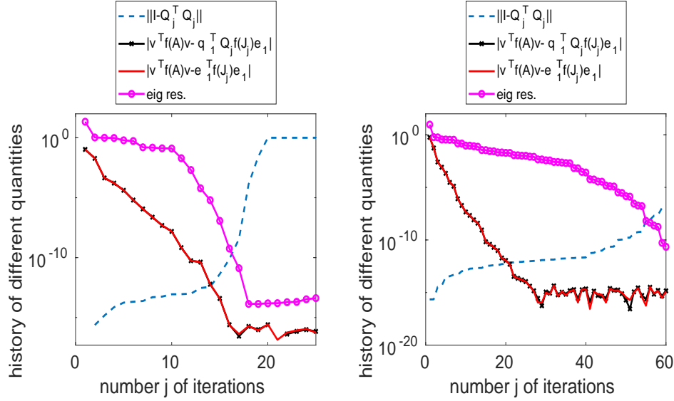
FIG. 4.1. Example 4.3. Convergence history of approximation to v^T A^{1/2} v . Left: \rho = 0.45 . Right: \rho = 0.85 .
