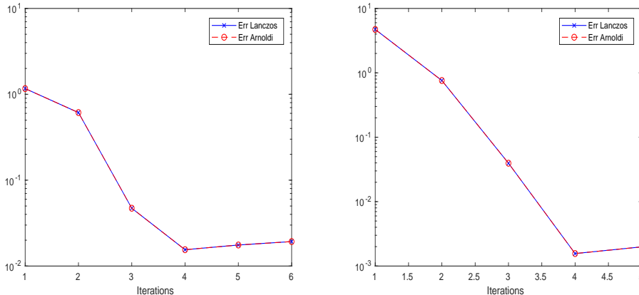
FIG. 3.2. Example 3.3. Convergence error history of the trace estimation (3.10) obtained at each step of the rational block Lanczos/Arnoldi methods.
