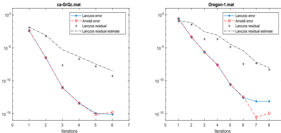
FIG. 3.1. Example 3.2. Convergence history of the Arnoldi error, together with the rational Lanczos error, residual norm (3.8) for \tau = 1 , and residual estimate (3.9).
