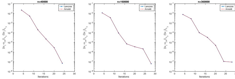
FIG. 3.3. Example 3.6. Convergence history of the rational Lanczos and Arnoldi methods for different values of n and s = 4 .
