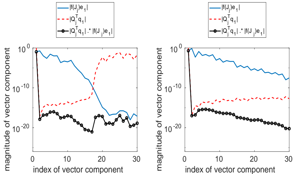
FIG. 4.2. Example 4.4. Magnitude of components at iteration j = 30 in the approximation to v^T A^{1/2} v . Left: \rho = 0.45 . Right: \rho = 0.85 .
