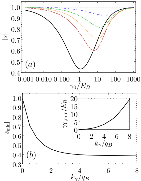
FIG. 4. (a) The S -matrix: |s(\mathbf{k}, \omega)| = |e^{i\delta(\mathbf{k}, \omega)}| as a function of the loss rate \gamma_0 (in units of E_B , computed at threshold \omega = \omega_{\text{th}} for k/q_B = 0.05 (solid black), 0.5 (dashed red), 1 (orange dotted), 2 (dotted-dashed green), 5 (double-dotted-dashed blue); here k_\gamma = 2.5q_B ). The dotted gray horizontal line is for infinitely fast losses, see Eq. (11). (b) The minimum of |s_{\min}| \equiv \min_{\gamma_0} |s(\gamma_0)| as a function of k_\gamma calculated for k = 0.05q_B . The inset of panel (b) shows the value of \gamma_0 for which |s| takes the minimum value, denoted by \gamma_{0,\min} . In both panels, m_c = m_f .
