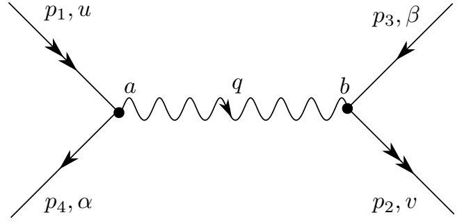
FIG. 9. The vertex generated by the action S_{\Delta c} , see Eq. (B24), describing interaction between a molecule ( \Delta , denoted with a solid line with a double arrow) and impurities (denoted with a solid line with a single arrow). Each line carries the momentum variable and the Keldysh index. The interaction mediated by fermions is denoted by the wavy line, which is labeled by a momentum variable q and two Keldysh indices (together they determine G_{f,ab}(q) ). To the diagram we assign the expression that is shown in Eq. (B25).
