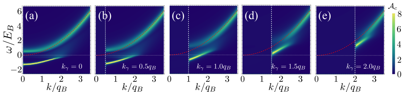
FIG. 2. Impurity spectral function \mathcal{A}_c(\mathbf{k}, \omega) (in units of E_B^{-1} ) as a function of |\mathbf{k}| and \omega (in units of q_B and E_B , respectively) for different sizes of the dissipative subspace: k_\gamma/q_B = 0, 0.5, 1.0, 1.5, 2.0 [from (a) to (e)]. The Fermi energy \epsilon_F = k_F^2/2m_f is set by k_F = q_B , and \gamma_0 = 20 E_B . The dotted horizontal line depicts \omega = 0 . The dashed vertical line [in the panels (b)–(e)] displays k_\gamma . The dashed red parabolic curve shows the dispersion relation \omega = k^2/2m_c of the free impurity.
