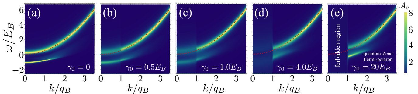
FIG. 1. The impurity spectral function \mathcal{A}_c(k, \omega) (in the units of E_B ) for a 2D system with the mass balance m_c = m_f . In the panels from (a)–(e) the strength of the loss is increased: \gamma_0/E_B = 0, 0.5, 1.0, 4.0, 20 . The energy is expressed in the units of the impurity-fermion binding energy E_B , and momenta are given in q_B = \sqrt{m_f E_B} . The Fermi energy \epsilon_F = k_F^2/2m_f is set by the Fermi wavevector k_F = 0.7q_B . The color coding of the values for \mathcal{A}_c is on the right. The cutoff momentum of the loss profile is at k_\gamma = q_B . The dashed red curve is the free dispersion relation \omega = \epsilon_c(k) \equiv k^2/2m_c .
