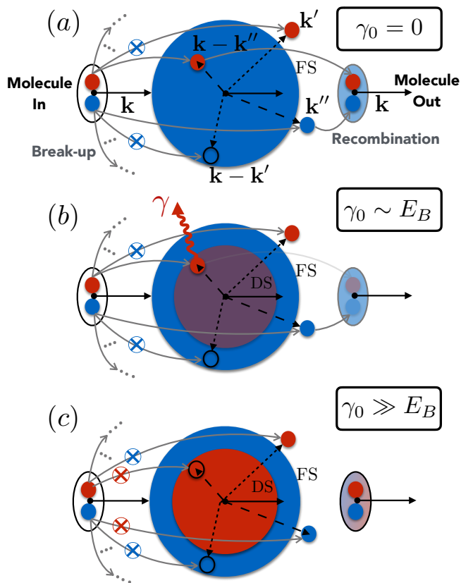
FIG. 3. The polaron is formed because the impurity (red circle) forms a molecular state with a fermion (blue circle). Crucially, the dynamics of molecules is in turn generated by virtual break-up processes followed by recombination, as illustrated here pictorially to complement the diagrammatic representation of Fig. 8b and the formal expression of Eq. (A9) for the molecular self-energy. A molecule with momentum \mathbf{k} temporarily breaks up into an impurity with momentum \mathbf{k}' and a fermion with momentum \mathbf{k} - \mathbf{k}' . The total effect is obtained by summing over all processes involving different momenta, as graphically indicated by the dots. In (a) the dissipationless case is considered, where the Pauli principle forbids processes creating a fermion within the Fermi surface (FS). In panel (b), moderate dissipation at a rate \gamma_0 comparable with the impurity-fermion binding energy E_B is added within the DS, which effectively makes the molecular state dissipative as well. Finally, in (c) the strongly dissipative regime is considered, where the quantum-Zeno effect forbids the creation of an impurity within the DS.
