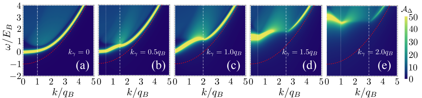
FIG. 6. Molecular spectral function \mathcal{A}_\Delta(\mathbf{k}, \omega) (in units of q_B^2 E_B ) for m_c = m_f as a function of |\mathbf{k}| (in units of q_B ) and \omega (in units of E_B ) for different sizes of the dissipative subspace: k_\gamma/q_B = 0, 0.5, 1.0, 1.5, 2.0 [from (a) to (e)]. The Fermi energy \epsilon_F = k_F^2/2m_f is set to k_F = q_B , and \gamma_0 = 20 E_B . The dotted/dotted-dashed vertical lines indicate |k_\gamma \mp k_F| . The dashed red curve is the molecular free dispersion given by \omega = -E_B + k^2/2M .
