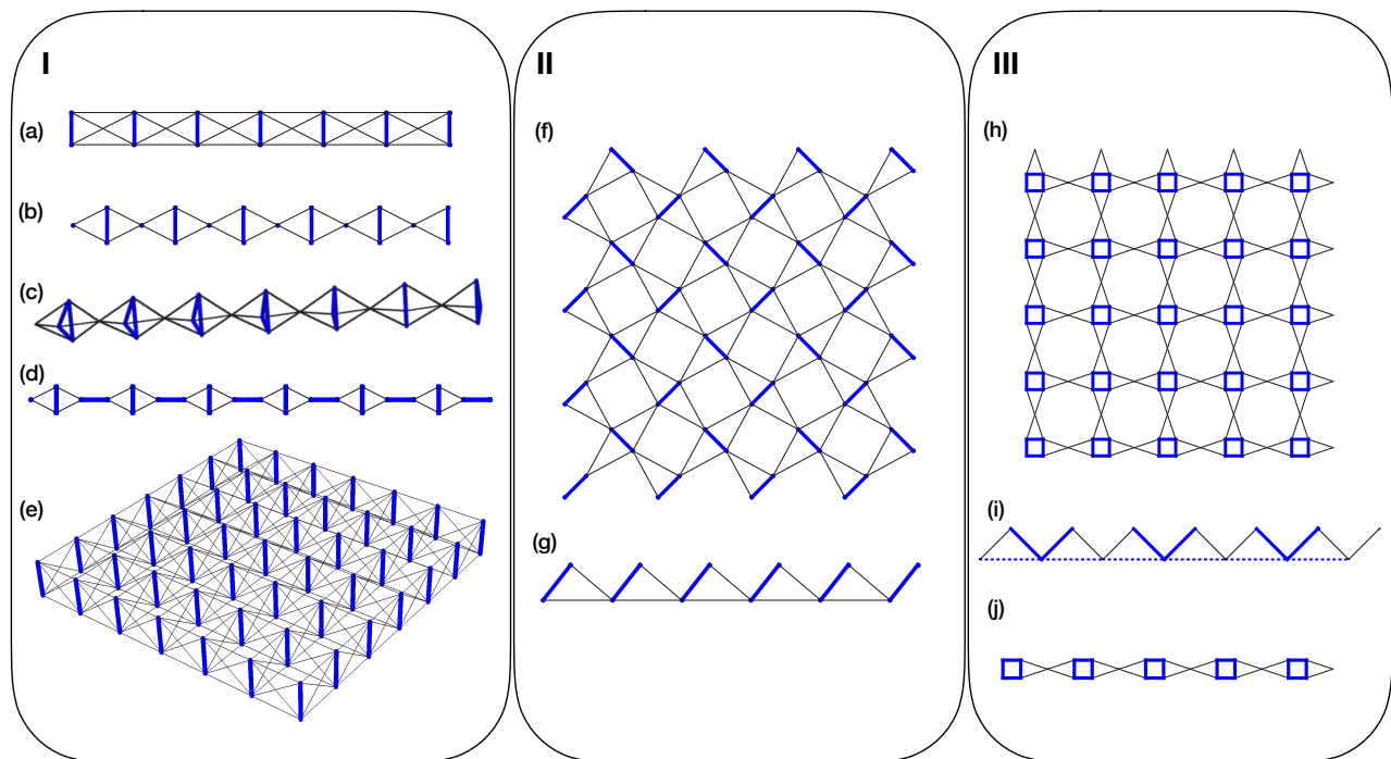
FIG. 1. Collection of lattices exhibiting athermal states in short-ranged interacting Heisenberg models with J couplings marked in thick blue and J' on the remaining bonds. Class (I): models on lattices (a)-(e) have an extensive number of local integrals of the motion. (a) Fully-frustrated ladder, (b) diamond chain, (c) pyrochlore chain, (d) orthogonal dimer chain, (e) fully-frustrated bilayer. Class (II) with protected singlet states: (f) Shastry-Sutherland lattice, (g) sawtooth chain with J bond on teeth. Class (III) with localized magnon states: (h) square kagome lattice (i) sawtooth chain with J' bonds on the spine (dotted), J bonds on every second valley which support the localized magnons (thick blue line) and J''=2J' on odd valleys (black solid line) and (j) the bowtie chain.
