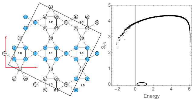
FIG. 8. (Left) Finite square kagome lattice of 30 sites used for the exact diagonalization study. The entanglement bipartition is indicated by the shading of the lattice sites. The exchange coupling J_n on the square plaquettes is shown for each square, while J' = 1.8 , \lambda = 0.5 throughout. (Right) Entanglement entropy within the total S^z = 22s sector on the 30 site system showing three scar states with zero entanglement entropy.
