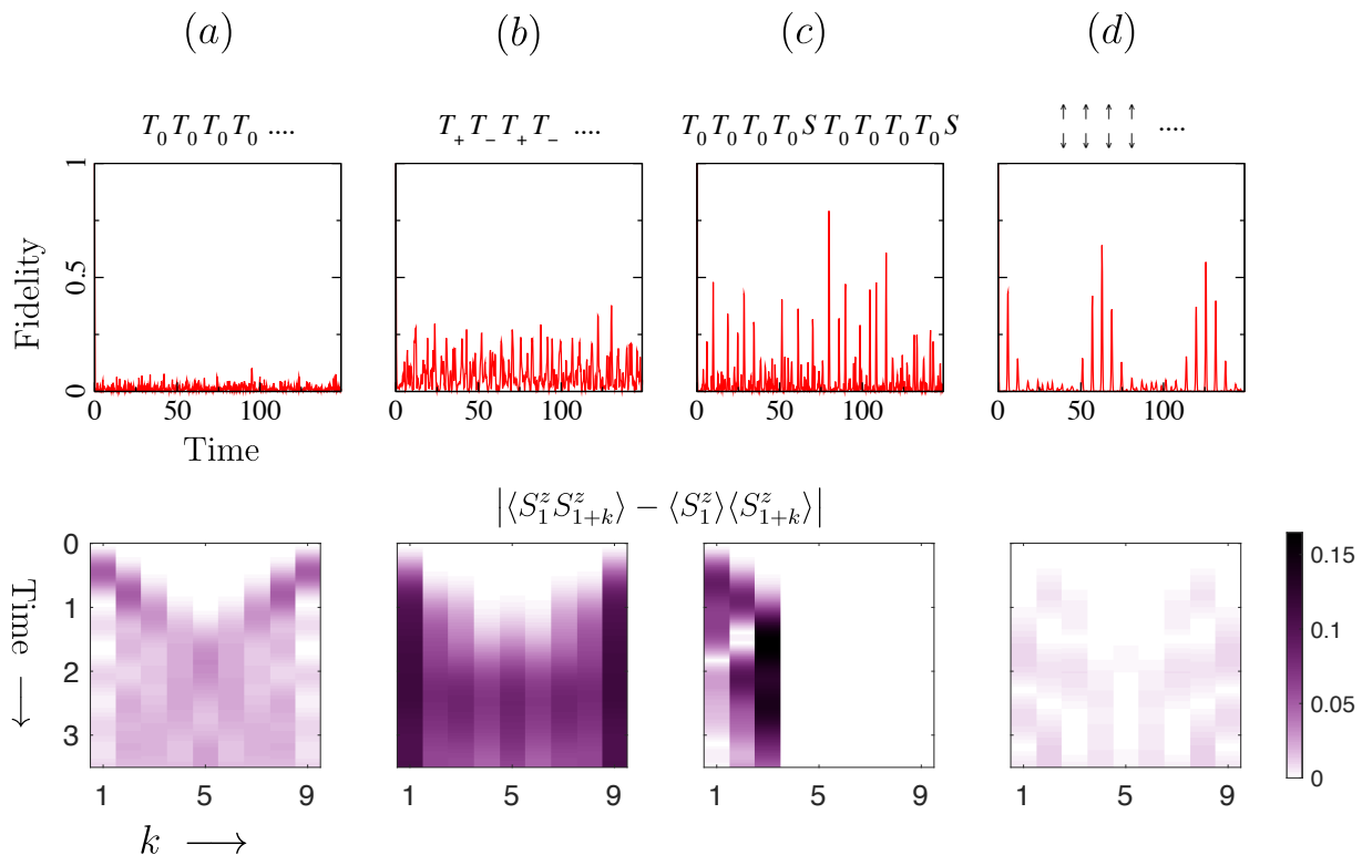
FIG. 3. Time evolution of the fully frustrated ladder with 10 rungs ( N = 20 , J = 1 , J' = 1.1 ), for four different initial states. Each column corresponds to a different initial state, as indicated. Upper row: fidelity |\langle\psi(0)|\psi(t)\rangle|^2 . Lower row: space-time density plots of the absolute value of the connected correlation function, \langle S_1^z(t)S_{1+k}^z(t)\rangle_c , between a spin on rung 1 and a spin on rung 1+k . Rung 1 is connected to rungs 2 and 10, corresponding to k = 1 and k = 9 , the rightmost and leftmost sites appearing in the density plots.
