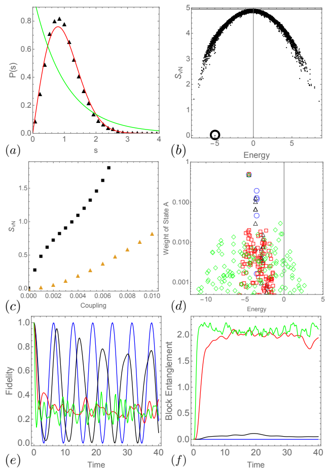
FIG. 5. Aspects of the sawtooth chain. (a) Level spacing statistics for N = 20 , J = 3 , J' = 1 , \lambda = -0.5 , compared with predictions for GOE (red) and Poisson (green). (b) Entanglement entropies in all eigenstates, for J = 1 , J' = 1.5 , \lambda = 0.5 , and N = 16 . Scar state is highlighted with a circle. The horizontal line at 4.949 is the random state entanglement for the (8, 8) bipartition. (c) Effect of perturbations on the entanglement of the scar state: J = 1.5 , J' = 1.0 , \lambda = 0.5 and J_p (squares), \eta (triangles). Dynamical signatures of scar states for an N = 12 chain: (d-f) J'/J = 0.05 (blue), J'/J = 0.5 (black), J'/J = 1.5 (red), J'/J = 4.5 (green). (d) Square of overlaps between the initial state (“state A”) and different eigenstates, plotted against eigen-energies. (e) The fidelity and (f) the block entanglement as functions of time.
