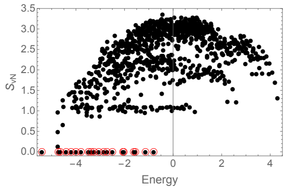
FIG. 6. Entanglement of the N = 12 sawtooth chain with open boundary conditions and entanglement cut in the middle of the chain (black points). The couplings are J = 1.0 and J' = 1.2 . The zero entanglement states for this cut have energies equal to those of the full spectrum on chain of length N = 6 (red circles) up to a constant shift.
