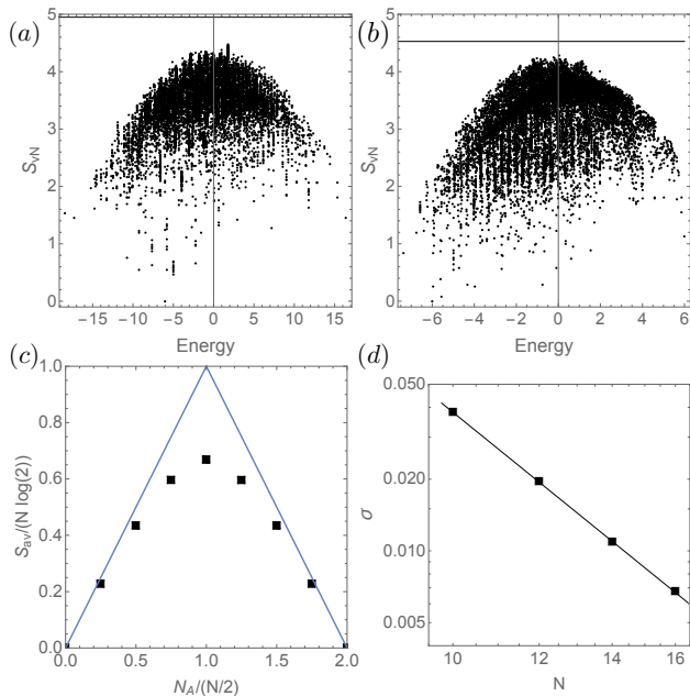
FIG. 2. Entanglement of eigenstates within total S^z = 0 sector, for two members of class (I). (a) Fully frustrated ladder, J = 1 , J' = 2 , \lambda = 0.5 , N = 16 ; an 8, 8 site bipartition. (b) Orthogonal dimer chain, J = J' = 1 , N = 16 ; a 9, 7 bipartition. The average entanglement of a random state with same Hilbert space size and same bipartitions is shown in each case as a horizontal line. Both plots show an anomalously broad distribution due to a large number of a conserved quantities. (c,d) are for the fully frustrated ladder. (c) Ratio of the average entanglement in the middle of the spectrum to the maximal entanglement as a function of the subsystem size N_A . Blue lines: envelope of maximal entanglement. (d) Scaling of the width \sigma of the distribution of off-diagonal matrix elements of a local operator, consistent with a power law \sigma \sim N^{-\alpha} and \alpha \approx 3.7 .
