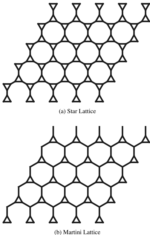
FIG. 4. Panels showing view in projection of lattices argued to belong to class of Heisenberg models with disorder-free localization. The full model is a bilayer of each of the above lattices with “fully frustrated” couplings between the two layers meaning that J couples the layers site-for-site and J' couples nearest neighbors within each layer and between layers. The “fully frustrated” square lattice bilayer is shown in Fig. 1 for reference.
