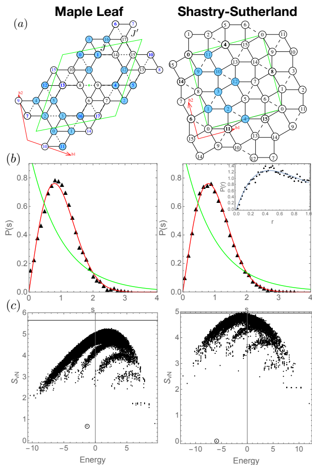
FIG. 7. Left column: Maple leaf lattice with 18 sites. Right column: Shastry-Sutherland lattice with either 20 sites (b) or 16 sites (a,c). (a) J ( J' ) bonds are dashed (full). One of the entanglement bipartitions is distinguished by blue shaded sites. The trapezoids demarcate the finite-size systems used for numerical diagonalization, with periodic boundary conditions. (b) Level spacing distributions, compared with Poissonian (green) and GOE (red) predictions. Left: maple leaf XXZ, J = 3 , J' = 1 , \lambda = -0.5 . Statistics from the middle 1/6th of the spectrum in the total S^z = 0 sector. Right: Shastry-Sutherland, N = 20 , J = 3 , J' = 1 , \lambda = 0 . Right inset shows distribution of ratios of level spacings. (c) Entanglement entropy of each eigenstate, against eigen-energies. Scar states are highlighted. The random state entanglement is indicated as a horizontal line in both panels. Left: maple leaf lattice, J = 0.2 , J' = 1 , \lambda = 0 . Right: Shastry-Sutherland lattice, N = 16 , J = 1 , J' = 1.25 , \lambda = 0 .
