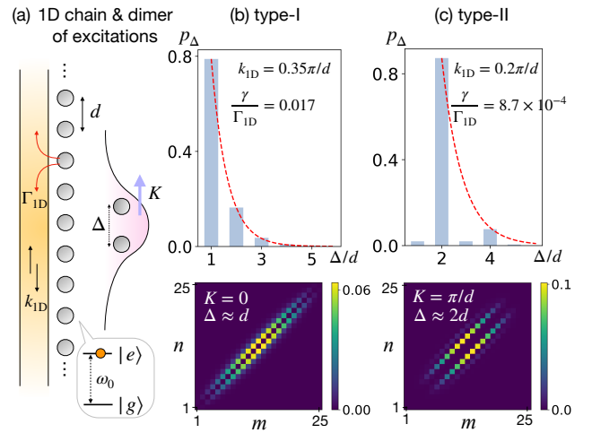
Figure 1. (a) A chain of two-level emitters couple to a 1D waveguide with parameters introduced in the main text. In the limit of infinite chains, a dimer state has two excitations characterized by a short relative distance \Delta and the delocalized “center of mass” (corresponding to a well defined total wave number K ). In this Letter we study two types of subradiant dimers: type-I states, dominated by K = 0 and \Delta = d , and type-II states dominated by K = \pi/d and \Delta = 2d . For finite chains of N=25 emitters, (b,c) show resonant examples of type-I and type-II dimers. Parameters of the resonant wave number and single emitter decay rates are specified in the upper panels which show the distribution of the separation \Delta between the excitations. The lower panels show the strongly correlated spatial distribution | \langle m, n | \psi \rangle |^2 of excited emitter pairs in the dimer states.
