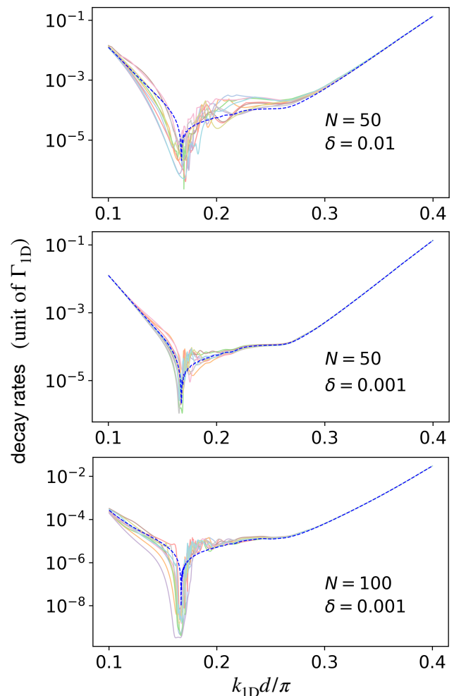
Figure 4. Effects of spatial disorder on the decay rates of the most subradiant type-II dimers, for different values of N and \delta displayed in the figures. In each subfigure, the blue dashed line corresponds to the case without disorder, and other lines show results for ten samplings of disordered chains.
