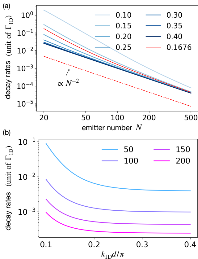
Figure 3. Decay rates of the most subradiant type-I dimer states. (a) Decay rates versus emitter number for values of k_{1D}d/\pi from 0.1 to 0.4 (every 0.05), and 0.1676. The dashed line is a guide to the eye for the N^{-2} scaling. (b) Decay rates versus k_{1D} for fixed N .
