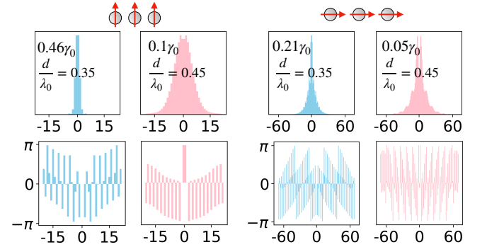
Figure 5. Bottom panels: phase profiles of the localized states discussed in the main text.
