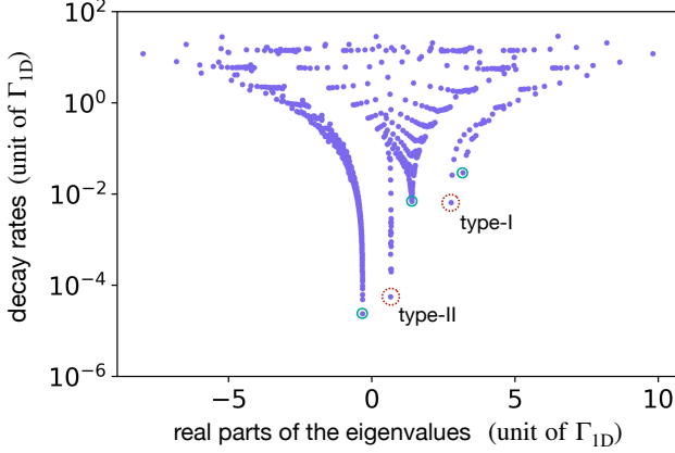
Figure 1. The eigenvalues of the two-excitation sector H_{\text{eff}} with N = 50 and k_{1\text{D}}d = 0.2\pi . Five branches of subradiant states are identified. Three of them are the fermionic states, of which the most subradiant ones are marked by green solid circles. The other two are the dimers. The most subradiant type-I and type-II are marked by red dotted circles.
