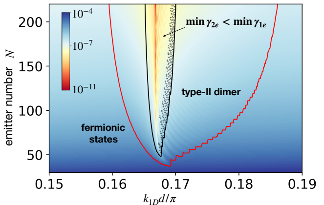
Figure 2. Decay rates of the most subradiant type-II dimers (shown by colors, with unit \Gamma_{1\text{D}} ) as function of emitter number N and lattice distance d . The red curve encloses the regime where the type-II dimers are longer lived than the fermionic states. The black line encloses the regime where the type-II dimers are even longer lived than the one-excitation states. In the shaded region, the dimer decay rate oscillates around the single excitation rates as function of N and d .
