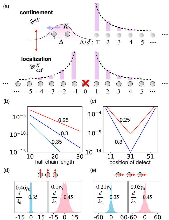
Figure 4. (a) The confinement of excitation pairs is equivalent to localization of an excitation around a missing site. (b) Decay rates (in units of \Gamma_{1\text{D}} ) of the state localized around the central missing site, for k_{1\text{D}}d/\pi = 0.25, 0.3, 0.35 . (c) Decay rates of the localized state as function of the position of the missing site in a chain with 60 emitters and k_{1\text{D}}d/\pi = 0.25, 0.3 . Profiles of the localized states of emitter chains coupled to free quantized field in 3D, with (d) transverse and (e) parallel polarization, for d = 0.35 and 0.45 times the resonant wavelength \lambda_0 . The decay rates are given in units of the single emitter spontaneous emission rate \gamma_0 .
