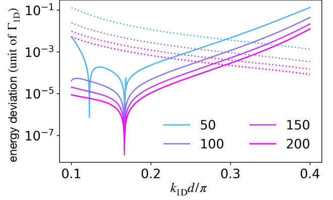
Figure 2. The dotted (solid) lines show the deviation between the real part of the eigenvalues (for finite chains) and the asymptotic eigenvalues \omega_{\text{I(II)}} , as function of k_{1\text{D}} for the type-I (type-II) dimers for different values of N .
