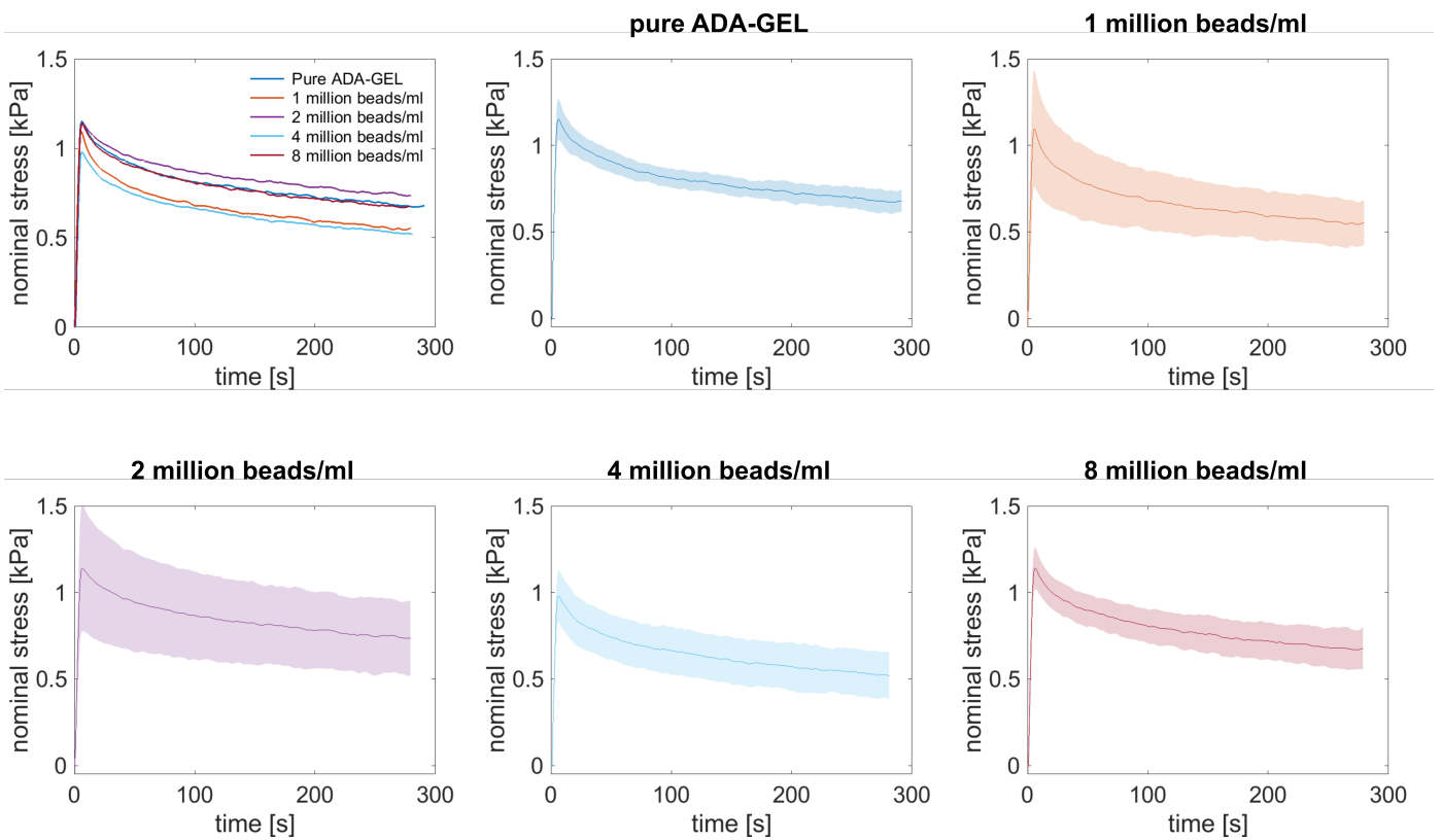
S 7: Stress relaxation behavior in tension for PAAm microgel bead-laden ADA-GEL samples with different bead concentrations.
