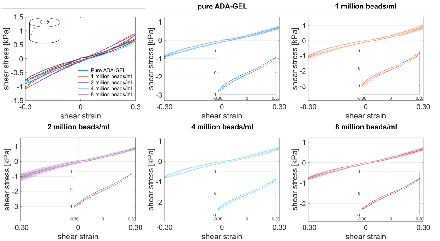
S 11: Response of PAAm microgel bead-laden ADA-GEL samples with different bead concentrations during torsional shear experiments up to a maximum shear of 30% .
