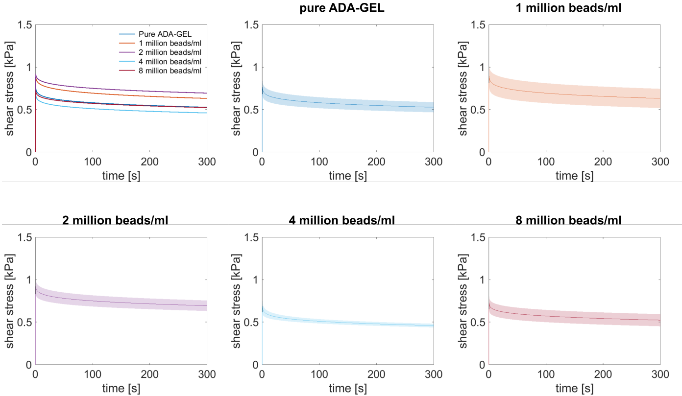
S 13: Stress relaxation behavior in torsional shear for PAAm microgel bead-laden ADA-GEL samples with different bead concentrations.
