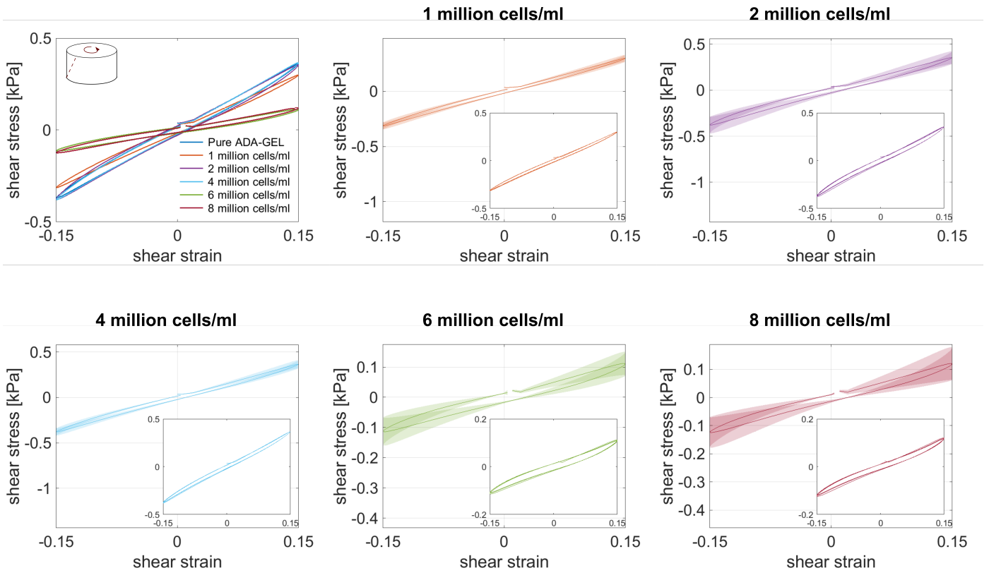
S 10: Response of cell-laden ADA-GEL samples with different cell concentrations during torsional shear experiments up to a maximum shear of 15% .
