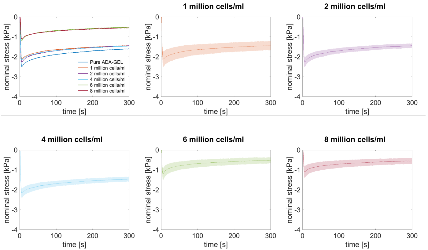
S 6: Stress relaxation behavior in compression for cell-laden ADA-GEL samples with different cell concentrations.
