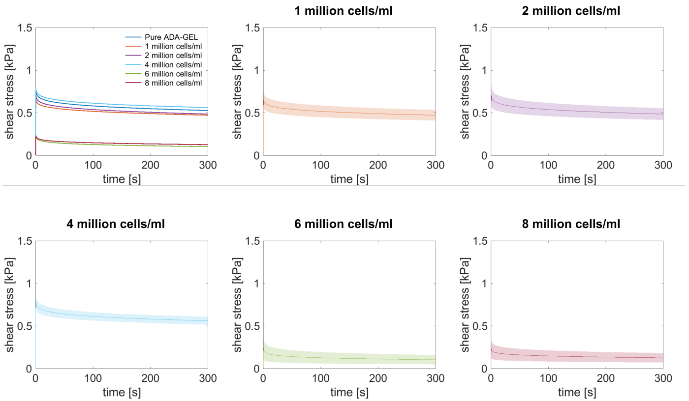
S 14: Stress relaxation behavior in torsional shear for cell-laden ADA-GEL samples with different cell concentrations.
