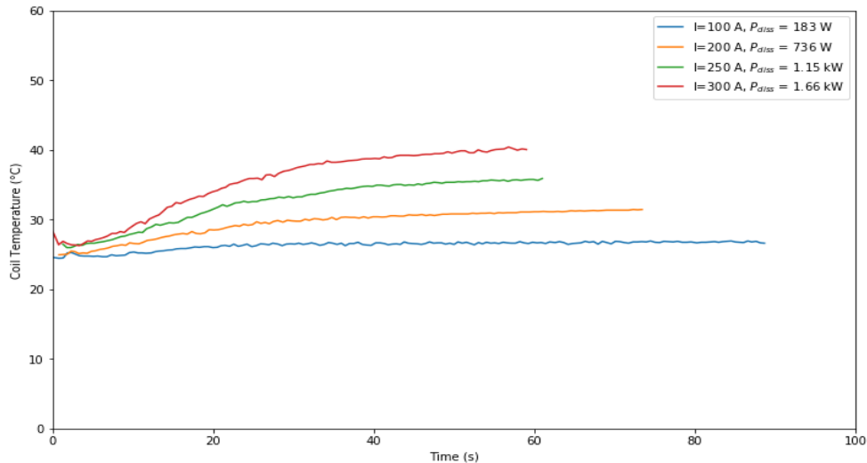
Figure 134: Temperature measurement of coil via Pt100 resistance for different dissipated powers.
