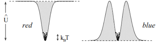
Figure 32: Needed radial intensity distributions for a red or blue detuned light field to have a trapping effect on e.g. the ground state of a two-level system. Figure taken from [42].
