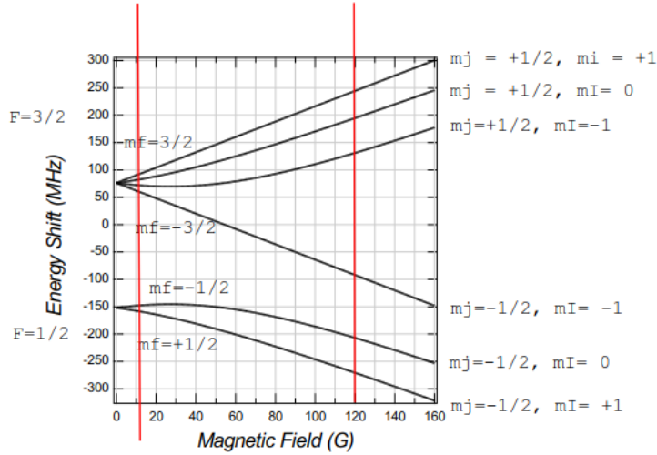
Figure 22: Magnetic-field dependence of the 2^2S_{\frac{1}{2}} ground state of {}^6\text{Li} . Taken, with slight modification, from [36].
