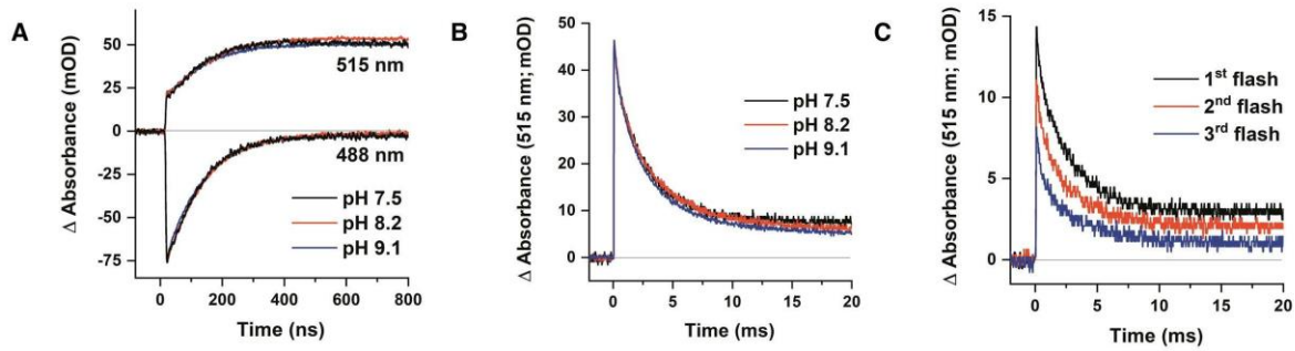
1 2 Fig. S10: Effects of pH and substrate consumption on the transient FAD absorption 3 changes in WT CvFAP.
