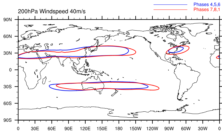
Figure 9. The 40\text{-m s}^{-1} contour is shown in blue averaged over MJO phases 4, 5, 6 and in red averaged over MJO phases 7, 8, 1 for the winter hemispheres, that is, DJF in the Northern Hemisphere and JJA in the Southern Hemisphere. MJO, Madden-Julian Oscillation; DJF, December, January, February; JJA, June, July and August.
