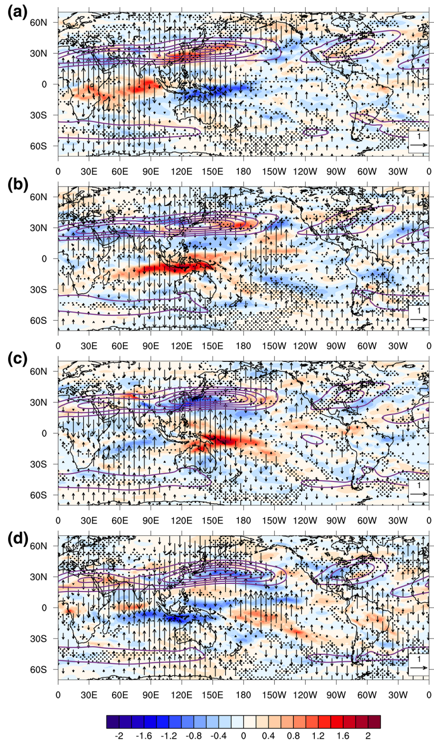
Figure 3. Meridional mass flux anomalies at 500 hPa (shaded, kg m -2 s -1 ) and the anomalous divergent meridional wind component at 200 hPa (arrows, m s -1 ) in (a)–(d) MJO phases 2, 4, 6, and 8 in DJF between 1979 and 2009. The purple contours show the total windspeed greater than 30 m s -1 , with the outermost contour representing 30 m s -1 , in intervals of 10 m s -1 at 200 hPa. The black stipples indicate regions where the meridional mass flux anomalies are not statistically different from the mean between 1979 and 2009 at the 95% confidence level. MJO, Madden-Julian Oscillation.
