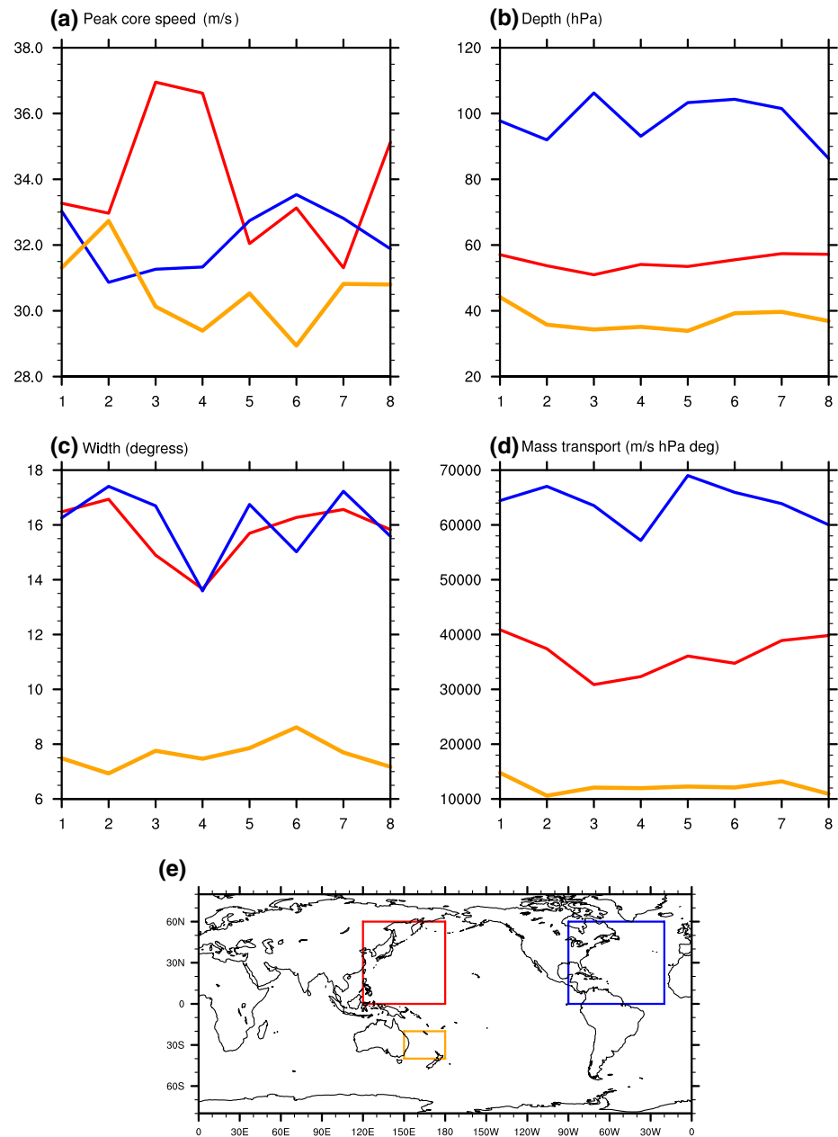
Figure 11. The same as in Figure 10 but for the summer hemispheres.
