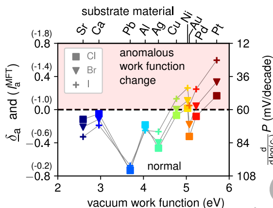
Figure 4. Numerical values for \delta_a and \mu_a^{\text{MFT}} = -(1 + \delta_a) for Cl, Br, and I on (111) surfaces of fcc metals, as derived from published theoretical data [74] (see section 7 in the SI). Positive and negative values of \delta_a classify systems according to their work function change (anomalous/normal) and are directly related to peak shifts \frac{d}{d \log(c_a)} P (eq. (36)) which we report on the right y-axis (Nernstian shift: \frac{d}{d \log(c_a)} P = 60 \text{ mV/decade} ).
