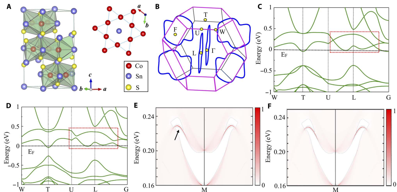
Fig. 1. Crystal and band structure of bulk single-crystal \text{Co}_3\text{Sn}_2\text{S}_2 . (A) Crystal structure of \text{Co}_3\text{Sn}_2\text{S}_2 obtained from single-crystal XRD and the Kagome lattice structure constructed by Co atoms in the a - b plane. (B) The 3D BZ projected in the (001) direction. Three pairs of nodal lines are shown in the first BZ. (C) Band structure of \text{Co}_3\text{Sn}_2\text{S}_2 in a paramagnetic state without the consideration of SOC effect. The band linear crossing near the Fermi energy can be found around the point L. (D) Band structure of \text{Co}_3\text{Sn}_2\text{S}_2 with the inclusion of SOC effect. The band linear crossing is open, resulting in the band gap. (E) The nontrivial surface states on (001) facet of \text{Co}_3\text{Sn}_2\text{S}_2 crystal with Sn termination, which is not fully occupied and located just above the Fermi level. (F) The contribution of Co atoms to the nontrivial surface states shown in (E). Nearly all the states originate from the surface Co Kagome layer.
