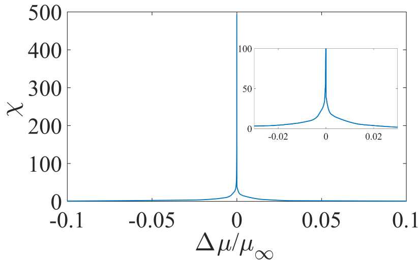
Figure 12: Susceptibility \chi calculated according to \chi = \mu^{-1} |\partial \mu / \partial S| vs reduced distance in control parameter \Delta \mu / \mu_\infty . The characteristic divergence at a critical point is clearly appreciated at the transition to chaos \Delta \mu = 0 .
