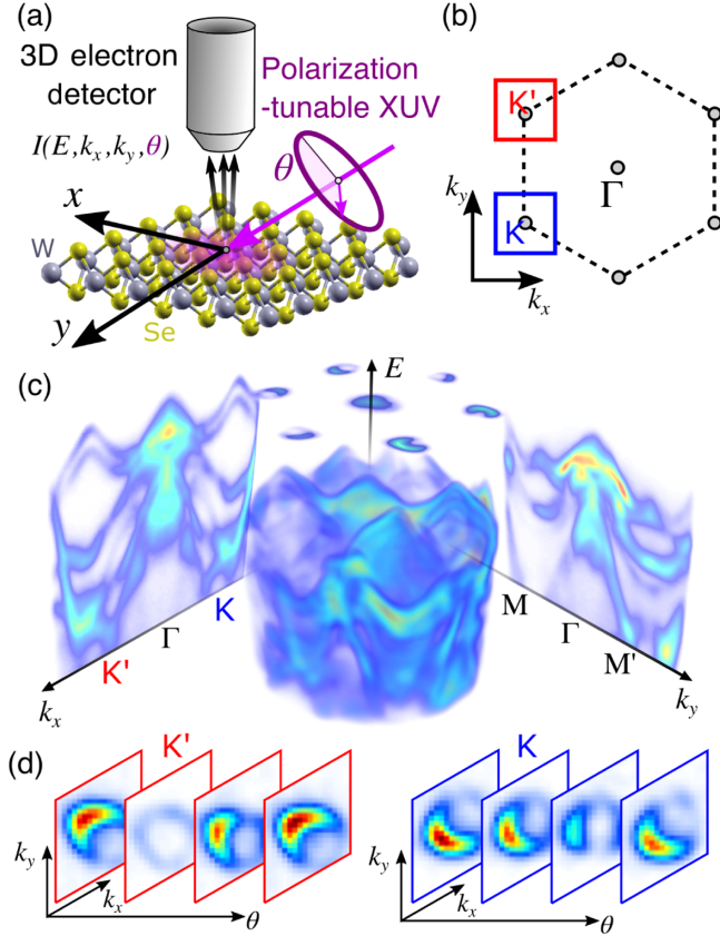
FIG. 1. Experimental setup and measurement protocol. (a) Experimental scheme of polarization-modulated, angle-resolved photoemission spectroscopy. A polarization-axis-tunable, linearly polarized, femtosecond XUV pulse (21.7 eV) is focused onto a bulk 2H-WSe 2 crystal at an angle of incidence of 65° with respect to the surface normal, ejecting photoelectrons that are detected by a time-of-flight momentum microscope, allowing us to measure the energy- and momentum-resolved photoemission intensity as a function of the polarization axis angle \theta — I(E, k_x, k_y, \theta) . (b) Sketch of the first Brillouin zone of 2H-WSe 2 . (c) Example of three-dimensional raw data—band structure mapping [ I(E, k_x, k_y) ] using p -polarized XUV radiation, an associated cut through high-symmetry directions ( K' - \Gamma - K and M' - \Gamma - M ), and a constant energy contour ( E - E_{\text{VBM}} = -0.25 eV). (d) Two-dimensional cut through the 4D ARPES intensity I(E, k_x, k_y, \theta) : at different polarization-axis angles ( \theta ), at E - E_{\text{VBM}} = -0.25 eV, and for given K and K' valleys.
