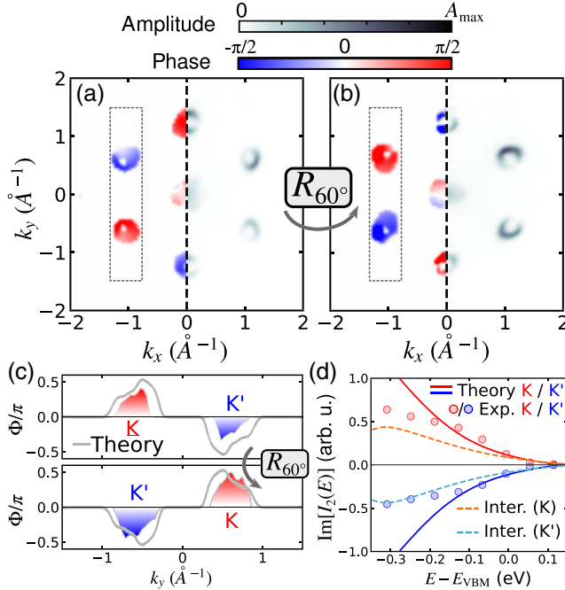
FIG. 4. Energy- and momentum-resolved Fourier analysis of the polarization-modulated ARPES signals. (a,b) Fourier amplitude |I_2(E, \mathbf{k})| (white-to-black color map, right subpanel) and phase \Phi(E, \mathbf{k}) (blue-to-red color map, left subpanel) of the photoemission modulation, for E - E_{\text{VBM}} = -0.25 eV. (c) Averaged phase [along a vertical cut and integrated over k_x as indicated by the dashed box in panels (a) and (b)] extracted from both the experimental data in panels (a) and (b) and the theory. (d) Valley-integrated imaginary part \text{Im}[I_2(E)] of the Fourier amplitude (5), comparing experiment and theory at K (red) and K' (blue), respectively. The dashed lines represent the corresponding interference contribution \text{Im}[I_2^{\text{int}}(E)] .
