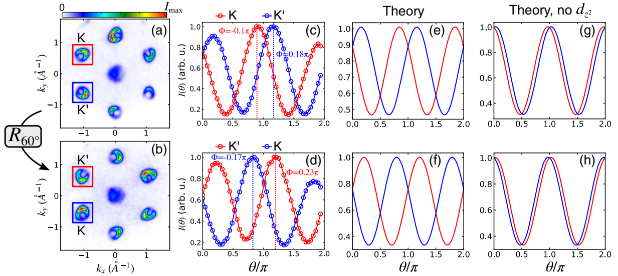
FIG. 3. Valley-resolved polarization-modulated photoemission. (a,b) Constant energy contours (binding energy E - E_{\text{VBM}} = -0.25 eV) for both crystal orientations (averaged over all polarization angles \theta ). (c,d) Valley-dependent polarization-modulated photoemission signal, integrated over the square boxes shown panels (a) and (b). The \theta dependence follows the generic form (2); the phase shift \Phi is illustrated by the dotted lines, and the value of \Phi for the K/K' valleys is given in the corresponding color. (e,f) Calculated polarization-angle modulation of the intensity [analogous to panels (c) and (d)]. (g,h) Analogous to panels (e) and (f), but excluding the |d_{z^2}\rangle orbital contribution. The direction of the light incidence is in the x - z plane.
