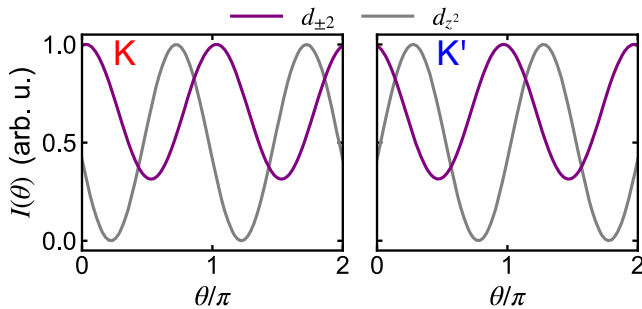
FIG. 7. Valley-integrated orbital-resolved photoemission intensity I_m(\theta) (analogous to Fig. 3) around the K and K' points, respectively [same as in Fig. 3(a)], for m denoting the d_{\pm 2} or the d_{z^2} orbital. The intensity has been normalized to the respective maximum.
