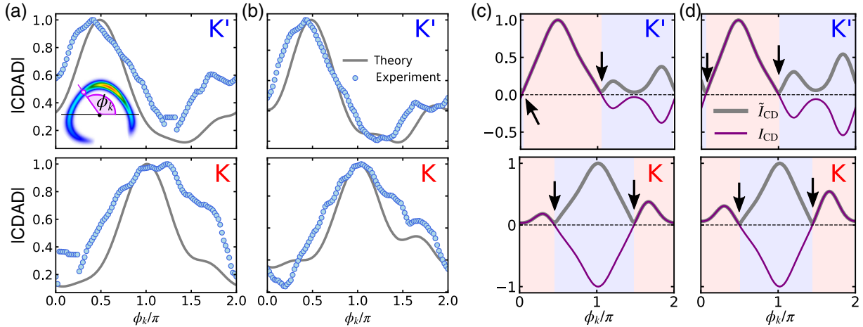
FIG. 5. Circular dichroism without circular photons. (a,b) Absolute value of the CDAD extracted from the experimental data and theory via Eq. (9) at fixed binding energy E - E_{\text{VBM}} = -0.18 \text{ eV} (a) and E - E_{\text{VBM}} = -0.25 \text{ eV} (b), as a function of the angle \phi_k tracing the intensity. The inset illustrates how the angle \phi_k is measured along the contour of maximum intensity. (c,d) Theoretical reconstructed [ \tilde{I}_{\text{CD}}(E, \mathbf{k}) ] and calculated CDAD [ I_{\text{CD}}(E, \mathbf{k}) ] as in (a,b). The arrows indicate the kink positions that can be used to determine sign changes (indicated by the shaded background).
