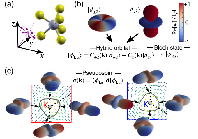
FIG. 2. Wave-function properties near the valence band maximum, around K/K' valleys. (a) Sketch of the crystal cell of a monolayer WSe 2 and the corresponding coordinate system (used for all three-dimensional plots in this figure). The purple arrows indicate the various polarization directions. (b) Relevant orbitals close to K/K' , represented by a constant-value surface of the absolute value. The color coding indicates the real part. The Bloch state |\psi_{\mathbf{k}\alpha}\rangle in the crystal cell in (a) is well approximated by a superposition of the |d_{\pm 2}\rangle and |d_{z^2}\rangle orbitals, which defines the hybrid orbital |\phi_{\mathbf{k}\alpha}\rangle . (c) Plots of the hybrid orbital of the top valence band at selected momentum points close to the K and K' [corresponding to the boxes in Fig. 1(b)] valley. There is a one-to-one map of the complex wave-function coefficients C_{0,\pm 2}(\mathbf{k}) forming the hybrid orbital and the orbital pseudospin \sigma(\mathbf{k}) ; the corresponding texture is represented by the vector field. The thick gray line is a contour of maximum photoemission intensity for typical binding energy.
