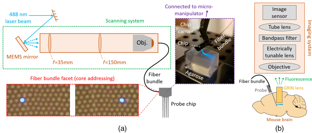
Fig. 2 Optical addressing method and proposal for deep-brain photonic-probe-enabled LSFM. (a) Schematic of the optical addressing method (not to scale). The scanning system addresses on-chip edge couplers via spatial addressing of the cores of an image fiber bundle. Bottom inset: micrographs of the distal facet of a fiber bundle connected to the scanning system with different cores addressed (adapted from Ref. 26). Top inset: annotated photograph of a packaged light-sheet neural probe inserted into an agarose block. (b) Illustration of the proposed use of the light-sheet neural probe with a GRIN lens endoscope for deep brain LSFM (not to scale). In this first investigation of the probe functionality, the configuration in (b) has not been demonstrated, and instead, the results here focus on a simpler imaging configuration where light-sheet probe illuminated samples are directly imaged with a fluorescence microscope without a GRIN lens (see Sec. 2).
