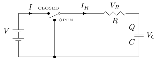
Figure 3 An RC circuit with a switch to disconnect the battery.
