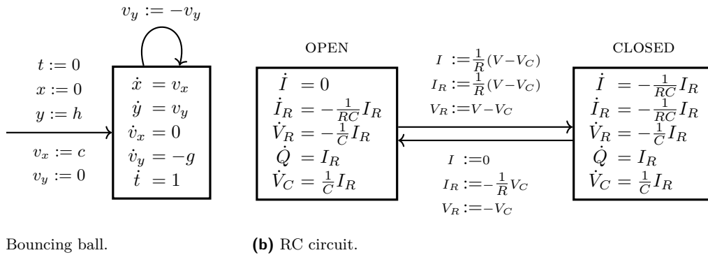
Figure 2 Examples of hybrid systems: (a) bouncing ball, (b) RC circuit.
