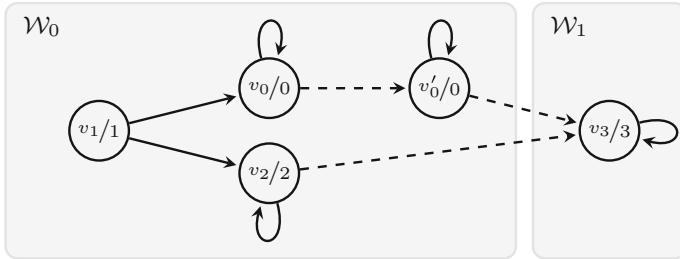
Fig. 8 A tradeoff between resilience and semantic quality (measured in the maximal color occurring infinitely often)
