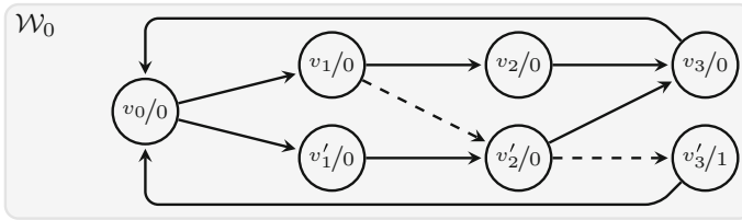
Fig. 6 Moving from v_0 to v_1 allows Player 0 to minimize visits to odd colors, while moving to v'_1 allows her to minimize the occurrence of disturbances
