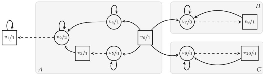
Fig. 1 A (max-) parity game with disturbances. Disturbance edges are drawn as dashed arrows. Vertices are labeled with both a name and a color. Vertices under control of Player 0 are drawn as circles, while vertices under control of Player 1 are drawn as rectangles
