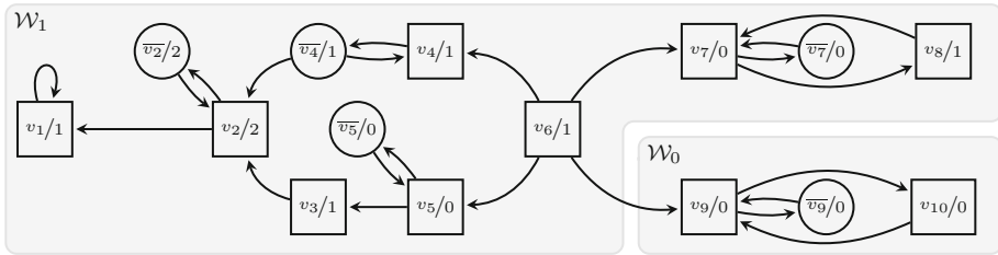
Fig. 2 The rigged game obtained for the game of Fig. 1
