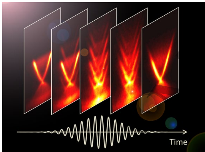
Fig. 1 Floquet-Bloch states observed on the Dirac-fermion surface state of a three-dimensional topological insulator, Bi 2 Se 3 [2]. Figure reprinted with permission from Fahad Mahmood.
