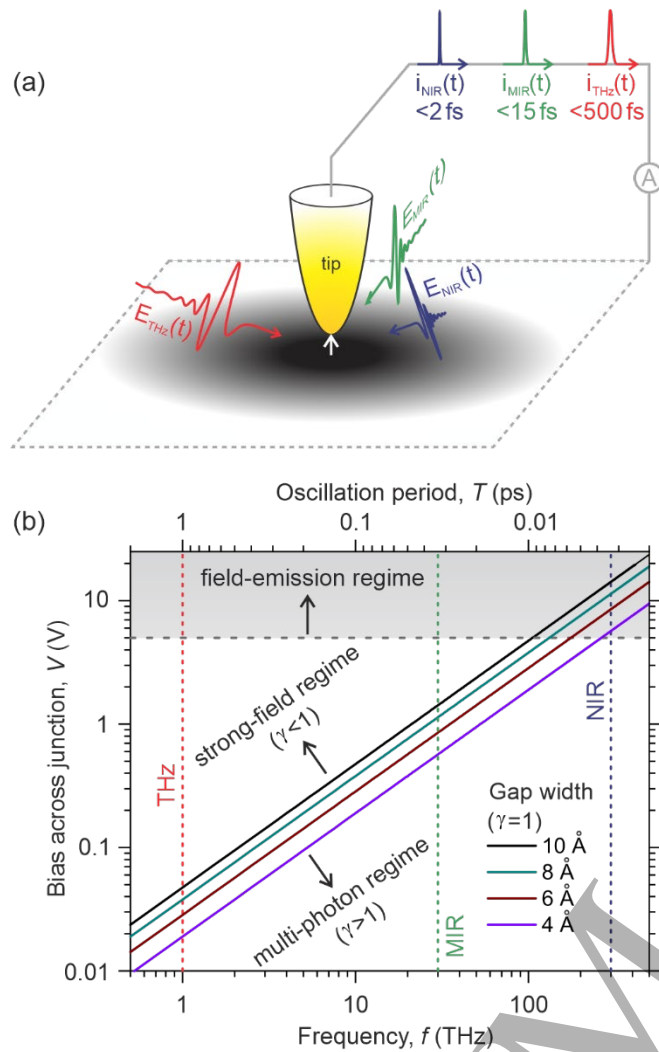
Figure 1. Lightwave-driven scanning tunnelling microscopy (LWD-STM) at different frequencies. (a) Experimental scheme: an ultrafast, phase-stable, single-cycle pulse in the terahertz (THz), mid-infrared (MIR) or near-infrared (NIR) spectral range is focused onto the tip of a scanning tunnelling microscope, where its field, E(t) , coherently controls the current across the tunnel junction. The nonlinearity of the tunnel junction leads to an asymmetric current pulse, i(t) , with a rectified component that can be detected by time-integrating electronics. The duration of the current pulse for unipolar tunnelling is less than half an oscillation cycle of the probe, defining the time resolution. The relative oscillation frequencies are not to scale. (b) The lightwave-driven tunnelling concept holds in the strong-field regime of optical nonlinearity, defined here as \gamma < 1 , where \gamma is the Keldysh parameter. Solid lines show voltages for which \gamma = 1 for different scanning tunnelling microscope tip heights. Above the work function of the sample ( \phi = 5 eV here, grey dashed line) the tunnel apparent barrier width becomes voltage dependent, corresponding to the field-emission regime (grey shaded region). The frequencies of the pulses in (a) are shown as vertical dashed lines (red: THz, 1 THz; green: MIR, 30 THz; blue: NIR, 300 THz). We note that for a constant input field the voltage applied across the junction is constant, i.e. it does not change with d [Jelic2017, Mueller2020], and emphasize that (b) is a conceptual map of the relevant LWD-STM regimes, not field enhancement.
