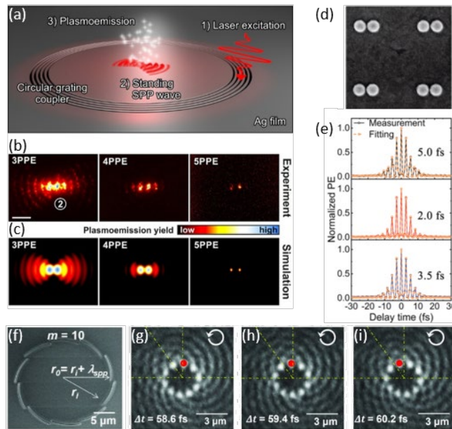
Figure 1. (a) Sketch of multiphoton plasmoemission from focused SPPs. (b) Energy-filtered plasmoemission based PEEM images of the focus spot at energies corresponding to different emission orders. (c) Corresponding simulation results. (d) Scanning electron microscope (SEM) image of nanodisk dimers. (e) Corresponding time-resolved photoemission intensities with fitted dephasing times, measured for different disk distances. (f) SEM image of a plasmonic Archimedean spiral lens (of the order m=10 ) for the generation of vortices with orbital angular momentum. (g-i) TR-PEEM images of a rotating plasmonic vortex within a single optical cycle. (a-c) is reprinted with permission from [2]. Copyright 2017 American Chemical Society. (d, e) is reprinted with permission from [7]. Copyright 2020 by the American Physical Society. (g-i) from [6]. Reprinted with permission from AAAS.
