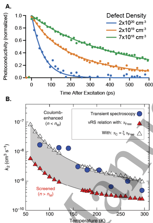
Figure 2. (A) An example of the variability of monomolecular recombination with defect density. For a series of formamidinium tin triiodide (FASnI 3 thin films), lifetimes of 59-590 ps are determined using optical pump/THz probe spectroscopy (OPTP) for defect densities ranging from 7 \times 10^{18} \text{ cm}^{-3} to 2 \times 10^{20} \text{ cm}^{-3} . The figure modified Milot et al. Adv Mater. 2018;30(44):1804506 and included in accordance with a Creative Commons Attribution licence. (B) Bimolecular recombination rate constant k_2 determined from OPTP measurements (blue circles) as compared to k_2 calculated via the van Roosbroeck-Shockley relation and fits to the steady-state absorption spectra. The figure is excerpted from Davies et al. Nat Commun. 2018;9:293 and reproduced in accordance with a Creative Commons Attribution licence.
