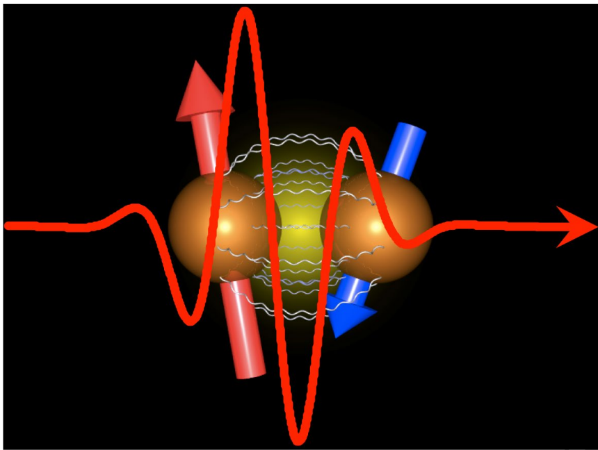
Figure 2. Pictorial view of the coherent interaction between spins and a single-cycle laser pulse (red solid line). The strong electric E field of the laser could modulate the exchange interaction and affect the spins orientation and magnitude via an E field-orbit-spin interaction or alternatively the laser pulse could couple to the spins via Zeeman interaction with the magnetic B field; such a coherent light-magnetic matter interactions should provide the ultimate time scales for spin manipulation with light.
