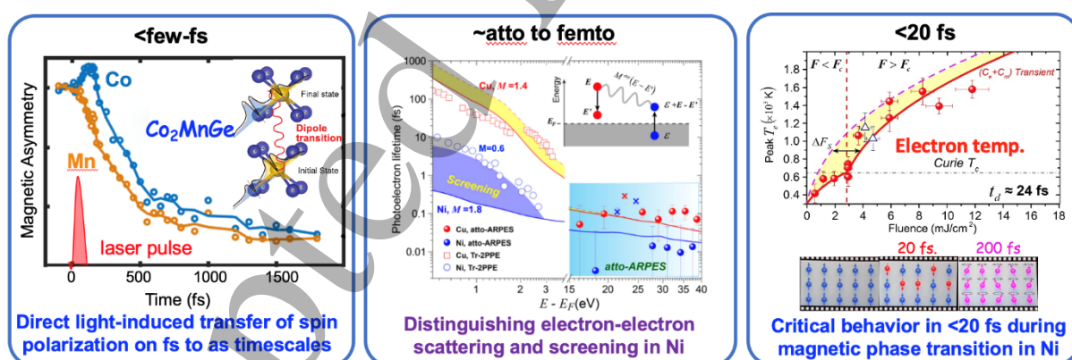
Figure 2. New timescales for spin manipulation observed experimentally. (left) Light can transfer spin polarization between two elements in a Heusler alloy, on few-fs timescales. Reprinted from [13]. © The Authors, some rights reserved; exclusive licensee American Association for the Advancement of Science. Distributed under a Creative Commons Attribution NonCommercial License 4.0 (CC BY-NC) http://creativecommons.org/licenses/by-nc/4.0/ . (centre) Distinguishing electron-electron scattering and screening in Ni. Reproduced with permission from [15]. (right) Ultrafast electron calorimetry showed that the energy required to drive a true magnetic phase transition in Ni is absorbed by the spin system within \sim 20 fs, clearly observable as an inflection point in the measured electron temperature at the Curie temperature. Reprinted from [4]. © The Authors, some rights reserved; exclusive licensee American
