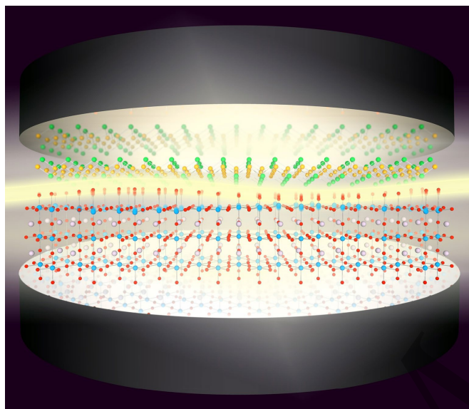
Fig. 2 Illustration of predicted cavity-controlled electron-phonon coupling and superconductivity in monolayer FeSe on SrTiO 3 substrate [8]. Figure courtesy: Jörg Harms, MPSD Hamburg.
