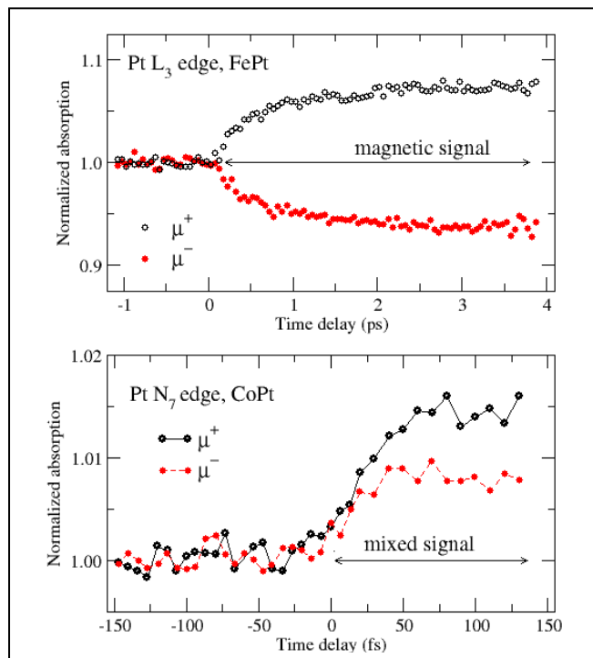
Figure 1. Comparison of pump-probe XMCD measurements of the time-resolved Pt magnetic moment in FePt (top) [4] and CoPt (bottom) [5]. The mirror symmetry around the \mu = 1 axis in the \mu^+ and \mu^- absorption coefficients at the Pt L_3 edge (top panel) represents a purely magnetic signal, attributed to ultrafast magnon generation [4]. The absence of mirror symmetry in the XMCD measurements at the Pt N_7 edge (bottom) signifies a significant charge response at noticeably short times, attributed to optical inter-site spin transfer from Pt to Co [5]. Note the different scales of the axes.
