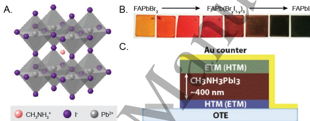
Figure 1. (A) Cubic crystal structure of methylammonium lead triiodide (CH 3 NH 3 PbI 3 ), the prototypical metal-halide perovskite. Hybrid metal halide perovskites demonstrate the classic AMX 3 perovskite structure, where A is an organic cation such as methylammonium or formamidinium, M is a divalent metal cation such as Pb 2+ or Sn 2+ , and X is a halide. (B) Thin films of mixed halide formamidinium (FA) lead perovskites demonstrating the tunability of the band gap with halide composition. Adapted from Eperon et al. Energy Environ Sci. 2014;7(3):982-8 with permission from the Royal Society of Chemistry. (C) A diagram of a perovskite solar cell. Light is absorbed by the perovskite layer and charge carriers then diffuse to the electron- and hole-transport media (ETM and HTM, respectively). The optically transparent electrode (OTE) typically consists of a conducting oxide layer deposited on glass, and a layer of gold serves as the counter electrode. This figure has been excerpted from Ref. (1) which can be accessed via https://pubs.acs.org/doi/abs/10.1021/acs.chemrev.6b00136 . Further permissions related to this material should be directed to the American Chemical Society.
