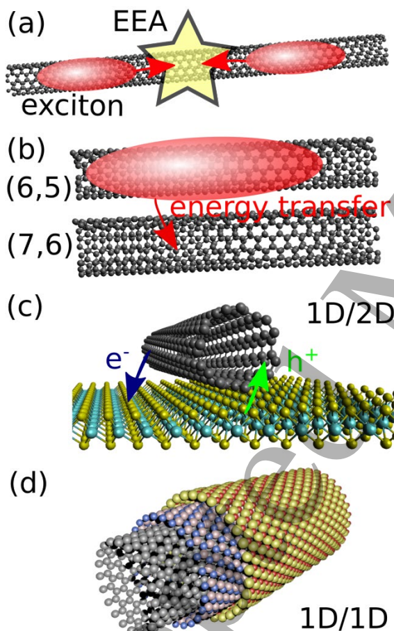
Figure 1 - (a) Exciton-exciton annihilation (EEA) in a carbon nanotube in the diffusion-limited regime. (b) Exciton energy transfer proceeding from a larger bandgap (6,5) CNT to a smaller gap (7,6) tube. (c) A mixed-dimension van der Waals heterostructure comprising a CNT bound to a transition metal dichalcogenide monolayer, creating a 1D/2D heterojunction. (d) A radial van der Waals heterostructure made from nanotube building blocks, forming 1D/1D heterojunctions.
